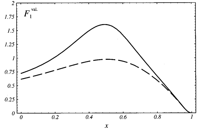
FIG. 7. As in Fig. 6, but for moderate binding for the model proton ( M = 1.8\bar{m} ).
