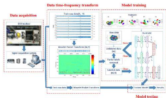
FIGURE 7. The framework of the proposed method for fault diagnosis of planetary gearbox [115].
