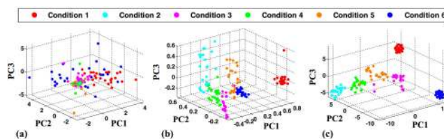
FIGURE 4. Three dimensional visualization of different features using PCA. (a) Compressed data features, (b) extracted 22 features, and (c) deep features [103].
