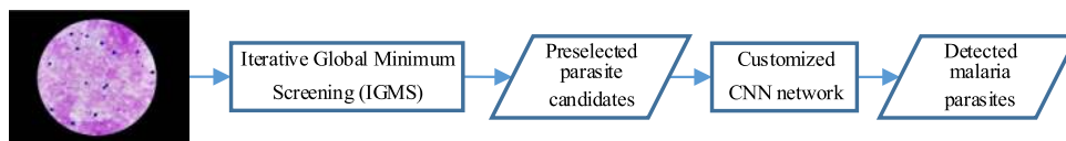
Fig. 2. Pipeline of the proposed system for automated parasite detection.
