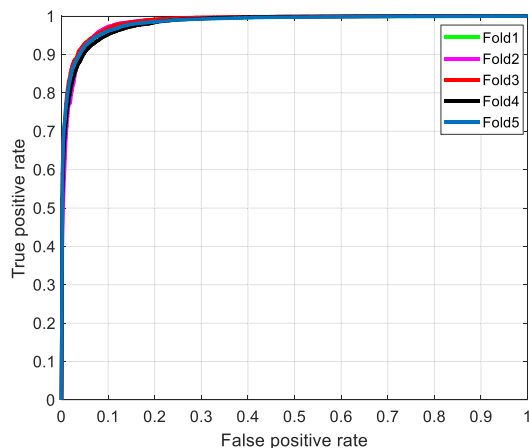
Fig. 11. ROC curves of the customized CNN model with five-fold cross evaluation for Set A on patch level (AUC = 98.39\% \pm 0.18\% ).
