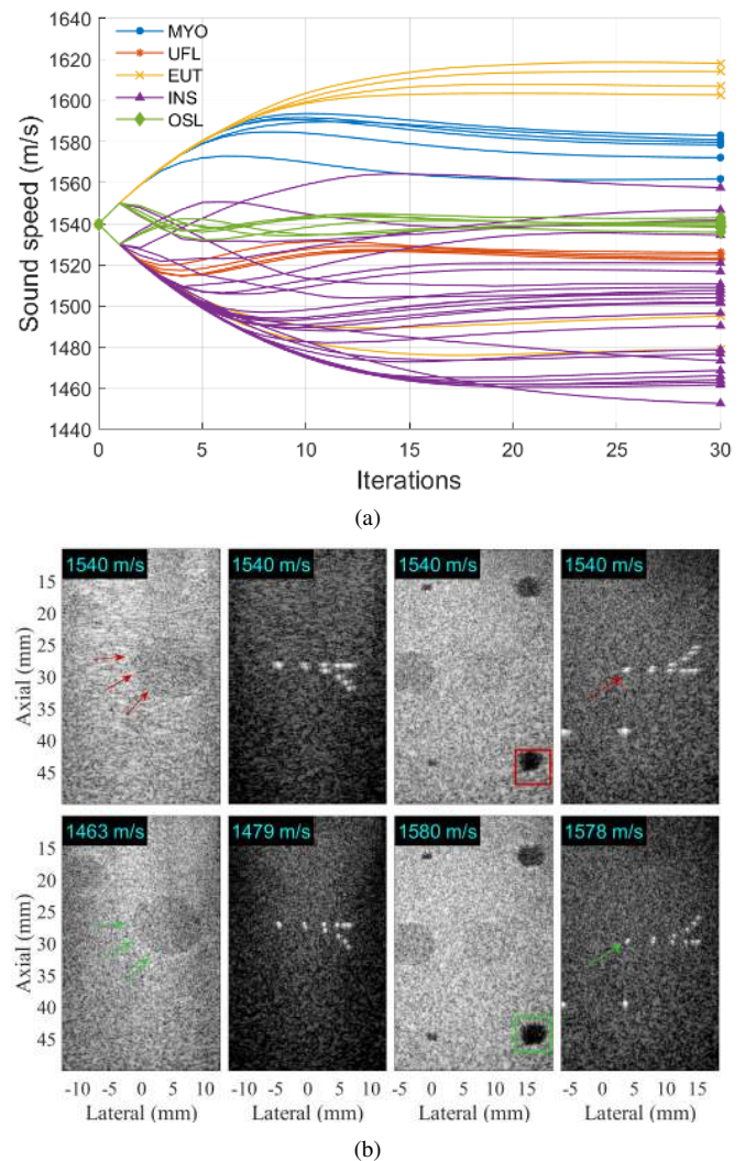
Fig. 1. (a) A wide range of optimal sound speeds were observed in contributed phantom datasets after 30 iterations of speckle brightness maximization. (b) Phantom images from sequences INS023, INS018, MYO001, and MYO003 are shown (from left to right, respectively) before (top) and after (bottom) global sound speed correction, displayed with 50 dB dynamic range. Arrows and boxes highlight locations where lesion boundaries are considerably sharper, point targets are visually more separable, and targets are repositioned to calibrated depths after sound speed correction.
