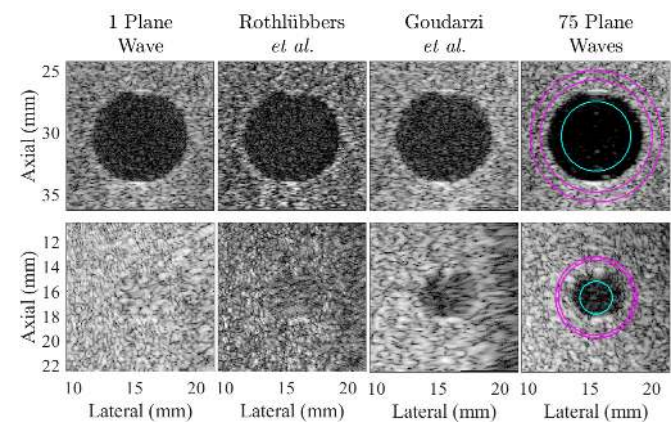
Fig. 3. Example results from the lesion test set, taken from dataset sequences UFL001 (top) and MYO001 (bottom), displayed with 40 dB dynamic range. The ROIs used for image quality metrics are overlaid on the 75 plane wave image, which served as the ground truth.
