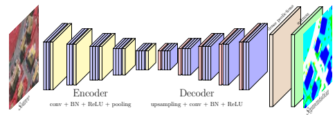
Fig. 3. Fully convolutional architecture for semantic labeling (SegNet [3]) of remote sensing data extracted from the ISPRS Vaihingen dataset.
