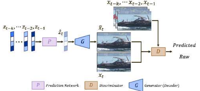
Figure 3. The latent space video prediction network estimates the next-frame latent with the understanding of latent space temporal correlation. A discriminator conditioned on the preceding frames provides feedback to the predictor so that it learns the mapping from the latent domain to the image space as well as the correlation of the previous and current frames. Given the sequence x_{t-k}, \dots, x_{t-1} , the actual x_t and predicted \tilde{x}_t are labeled as real and fake samples for the discriminator. As such, the predictor adversarially learns the temporal correlation.
