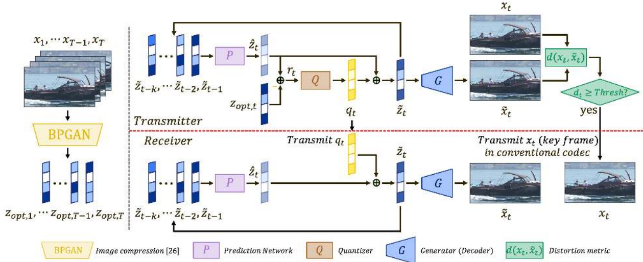
Figure 2. The operational flow of our proposed codec. Each frame of the video sequence is first individually compressed to a latent representation by the method in [26]. The predicted next-frame latent (output of the prediction network) is conditioned on the former reconstructed latent representations. The data we store and transmit is the quantized and entropy coded residual q_t . The transmitter and the receiver share the same prediction network, which produces identical reconstructed latents \tilde{z}_t on both sides. \tilde{z}_t is fed to the prediction network to estimate future frames, and to the generator to decode the video frame \tilde{x}_t . To preserve the quality of the reconstructed data sequences, we monitor the distortion between the original and reconstructed frames on the transmitter side, and directly send the encoded original key-frame to the receiver only if the distortion is above a certain threshold.
