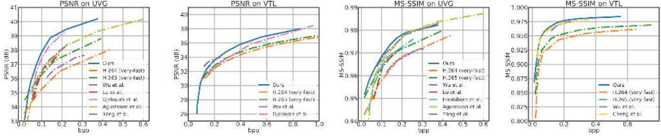
Figure 4. Comparison of our proposed approach with H.264, H.265, and learning-based codecs [50, 31, 15, 51, 3] for PSNR, and [50, 31, 19, 12, 51, 3] for MS-SSIM on UVG and VTL datasets. Our video codec is not optimized specifically for PSNR or MS-SSIM.
