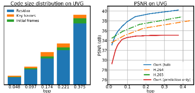
Figure 6. Code length distribution for different compression ratios (left) and evaluation of next-frame prediction performance (right). The prediction-only method generates the video sequences from predicted next-frame latents \hat{z}_t without residual compensation whereas the input to the predictor is the reconstructed latents \tilde{z}_t . Note that bpp values for the prediction-only curve do not reflect the actual code size (which should be very close to 0 as residuals are discarded). They are just proportional to the latent space dimension we adopted for the experiment.
