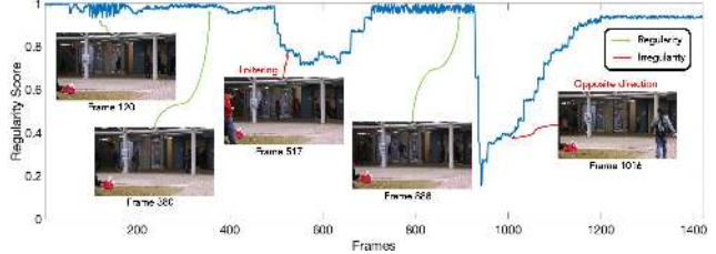
Figure 7. Regularity score (blue curve in the figure) along the frame sequence. Normal scenes typically score > 0.9 whereas abnormal events cause steep score degradation.
