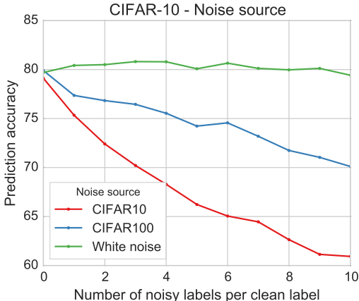
Figure 6: Performance on CIFAR-10 for varying amounts of noisy labels. Noisy training examples are drawn from (1) CIFAR-10 itself, but mislabeled uniformly at random, (2) CIFAR-100, with uniformly random labels, and (3) white noise with mean and variance chosen to match those of CIFAR-10. Noise drawn from CIFAR-100 resulted in only half the drop in performance observed with noise from CIFAR-10 itself, while white noise examples did not appreciable affect performance.
