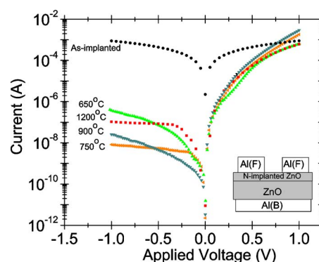
FIG. 1. (Color online) I - V data of the N^+ -implanted undoped MG ZnO samples with different postimplantation annealing temperatures in air. The I - V measurements were performed across the Al(F)-Al(B) connection.
