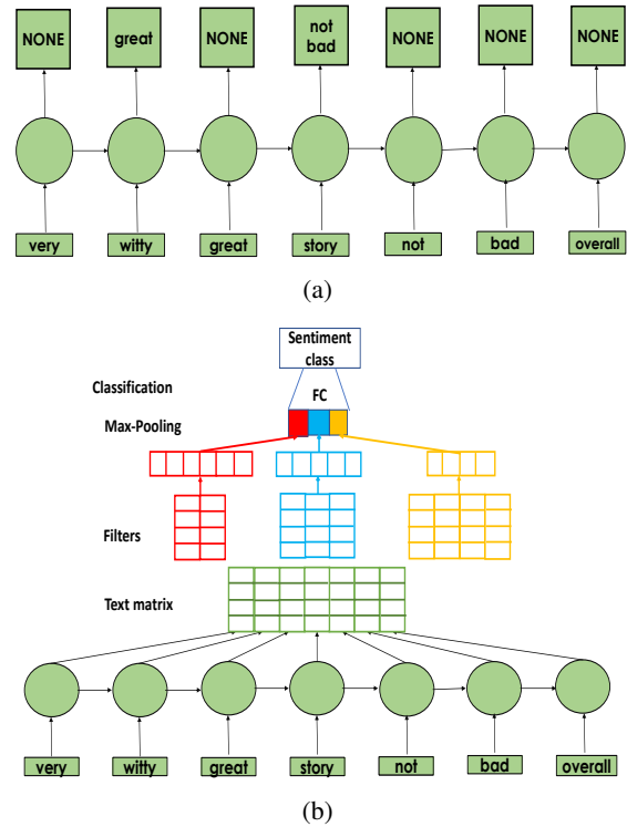
Figure 2: The PBLM model (figure imported from ZR18). (a) The PBLM representation learning model. (b) Adapting a classifier with PBLM: the PBLM-CNN model where PBLM representations are fed into a CNN task classifier.
