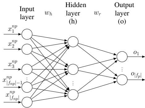
Figure 1: The AE-SCL and AE-SCL-SR models (figure imported from ZR17). x^{np} is a binary vector indicating whether each of the non-pivot features appears in the input example. x^p is a similar vector defined with respect to pivot features. o , the output vector of the model, provides the probability that each of the pivot features appears in the example. The loss function of both models is the cross-entropy loss between o and x^p . While in AE-SCL both the encoding matrix w^h and the reconstruction matrix w^r are optimized, in AE-SCL-SR w^r consists of pre-trained word embeddings.
