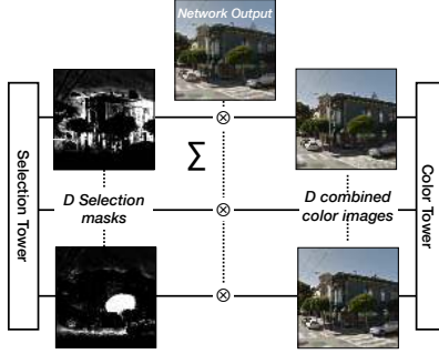
Figure 3: The basic architecture of our network, with selection and color towers. The final output image is produced by element-wise multiplication of the selection and color tower outputs and then computing the sum over the depth planes. Fig. 6 shows the full network details.
