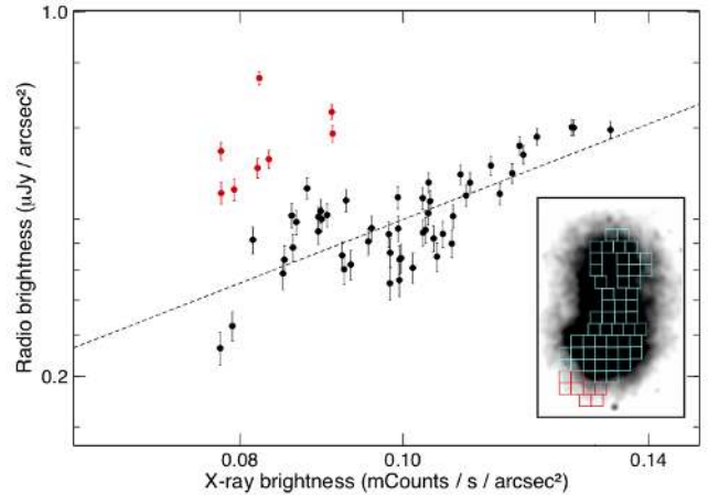
FIG. 18.— I_{\text{radio}} - I_{\text{X-ray}} relation of the 1RXS J0603.3+4214 cluster. The error-bars represent the RMS of the brightness distribution within each cell. The power-law fit is indicated by a dashed line. Red and cyan boxes, overlaid on the Chandra X-ray image, show the regions where the radio and X-ray surface brightness were extracted. We exclude regions where there is a point source. The surface brightness extracted in cyan cell are indicated by black dots. The red dots are extracted across the southernmost part of the radio halo, i.e. the region between the cold front and the southern shock front, shown with red regions. As discussed in Section 5.5, the southern part of the radio halo may have a different origin than the rest of the halo.
