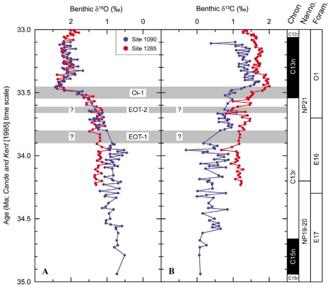
Figure 3. ODP Sites 1090 and 1265 benthic foraminiferal stable isotope records across the Eocene-Oligocene transition. (a) Sites 1090 (blue circles) and 1265 (red circles) benthic foraminiferal ( Cibicidoides spp.) \delta^{18}\text{O} data versus age in millions of years. (b) Sites 1090 and 1265 benthic ( Cibicidoides spp.) foraminiferal \delta^{13}\text{C} data. Oxygen and carbon isotope values are reported relative to the VPDB (Vienna Pee Dee belemnite) standard. Gray bars mark the EOT-1 (Eocene-Oligocene transition event 1), EOT-2 (Eocene-Oligocene transition event 2), and Oi-1 (Oligocene isotope event 1) events occurring at 33.8, 33.63, and 33.54 Ma, respectively [Miller et al., 1991, 2008; Lear et al., 2004; Coxall et al., 2005; Katz et al., 2008]. The biomagnetostratigraphic age model follows Berggren et al. [1995], Cande and Kent [1995], and Berggren and Pearson [2005].
