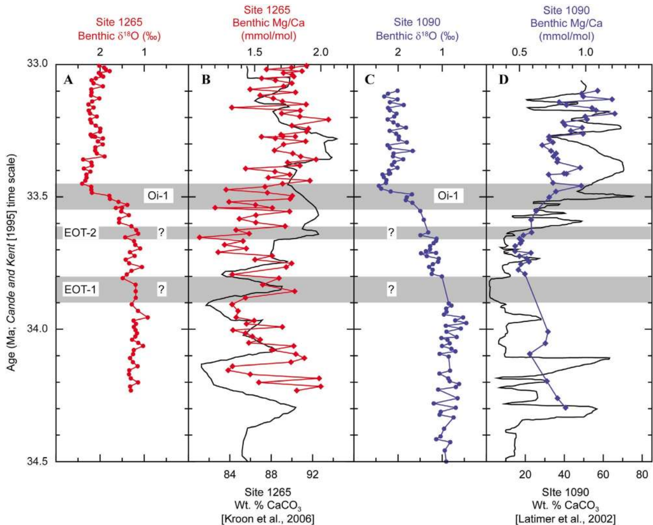
Figure 5. ODP Sites 1265 and 1090 benthic foraminiferal \delta^{18}\text{O} , Mg/Ca, and weight percent carbonate records versus age in millions of years. (a) Site 1265 benthic foraminiferal \delta^{18}\text{O} values (red circles; Cibicidoides spp.) versus age in millions of years. Isotope values are reported relative to the VPDB (Vienna PeeDee belemnite) standard. (b) Site 1265 benthic foraminiferal Mg/Ca ratios (red diamonds; C. praemundulus ) in mmol/mol plotted with weight percent carbonate (black line) from Kroon et al. [2006]. (c) Site 1090 benthic foraminiferal \delta^{18}\text{O} values (blue circles; Cibicidoides spp.). (d) Site 1090 benthic foraminiferal Mg/Ca ratios (blue diamonds; Cibicidoides spp.) in mmol/mol plotted with weight percent carbonate (black line) from Latimer and Filippelli [2002]. Gray bars mark the EOT-1 (Eocene-Oligocene transition event 1), EOT-2 (Eocene-Oligocene transition event 2), and Oi-1 (Oligocene isotope event 1) events occurring at 33.8, 33.63, and 33.54 Ma, respectively [Miller et al. , 1991, 2008; Lear et al. , 2004; Coxall et al. , 2005; Katz et al. , 2008].
