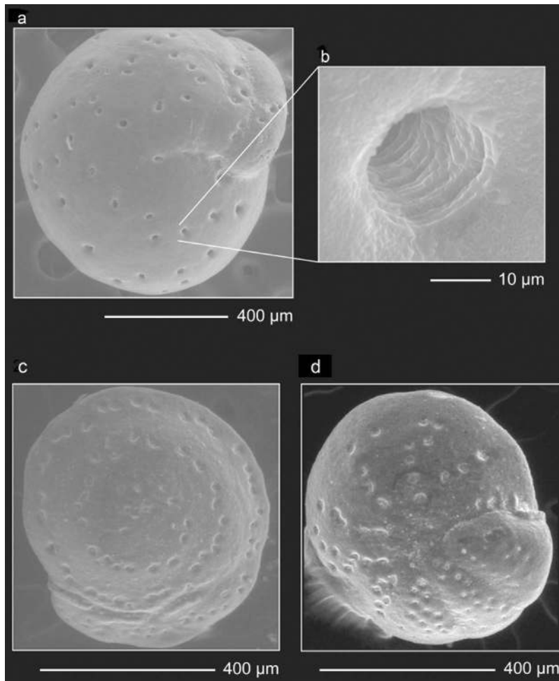
Figure 2. SEM images of Ocean Drilling Program Sites 1090 and 1265 benthic foraminiferal specimens from the genus Cibicoides at 228.24 and 186.58 m composite depth (mcd), respectively. (a) ODP Site 1090 Cibicoides grimsdalei SEM image at 400 \mu\text{m} from 228.24 mcd with 30 weight percent \text{CaCO}_3 [Latimer and Filippelli, 2002]. (b) ODP Site 1090 Cibicoides grimsdalei SEM image at 10 \mu\text{m} from 228.24 mcd with 30 weight percent \text{CaCO}_3 [Latimer and Filippelli, 2002]. (c) ODP Site 1265 Cibicoides praemundulus SEM image at 400 \mu\text{m} showing spiral side of foraminifera from 186.58 mcd with 85 weight percent \text{CaCO}_3 [Kroon et al., 2006]. (d) ODP Site 1265 Cibicoides praemundulus SEM image at 400 \mu\text{m} showing umbilical side of foraminifera from 186.58 mcd with 85 weight percent \text{CaCO}_3 [Kroon et al., 2006].
