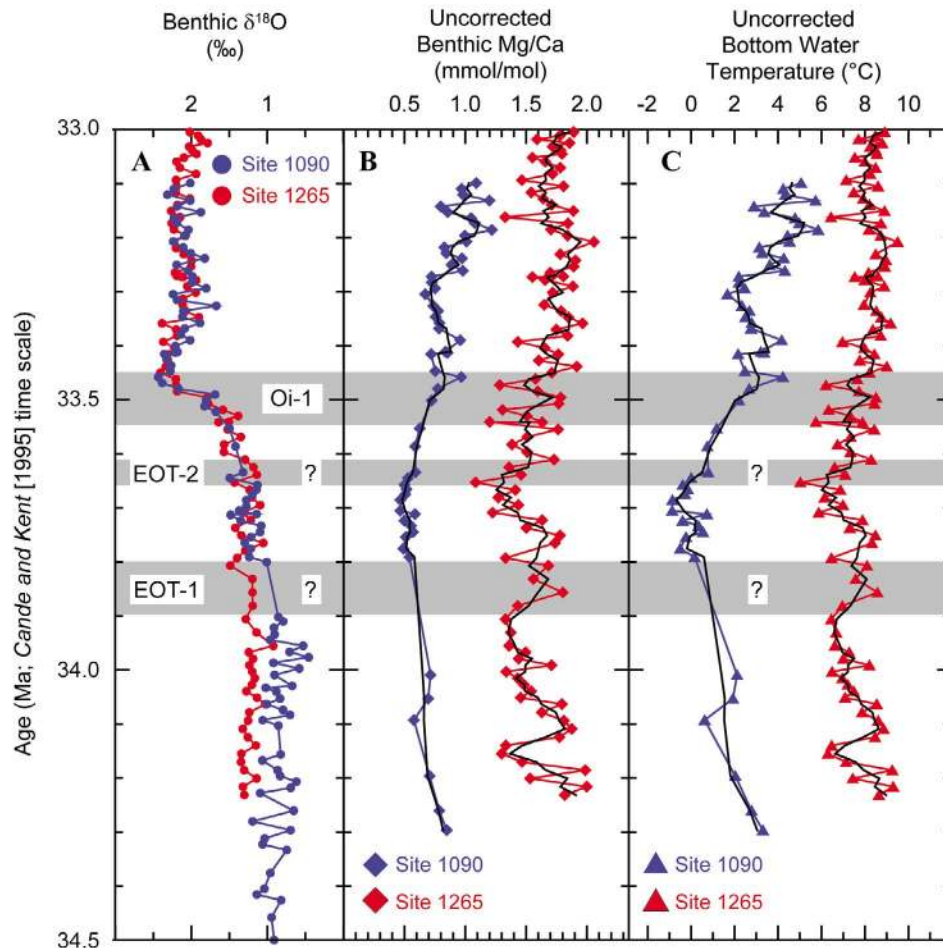
Figure 7. ODP Sites 1090 and 1265 benthic foraminiferal \delta^{18}\text{O} , uncorrected Mg/Ca, and uncorrected bottom water temperature (BWT) records versus age in millions of years. (a) Benthic foraminiferal ( Cibicidoides spp.) \delta^{18}\text{O} records from Sites 1090 (blue circles) and 1265 (red circles). Isotope values are reported relative to the VPDB (Vienna PeeDee belemnite) standard. (b) Sites 1090 (blue diamonds; Cibicidoides spp.) and 1265 (red diamonds; C. praemundulus ) benthic foraminiferal Mg/Ca ratios in mmol/mol uncorrected for changes in the deep water carbonate ion concentration associated with Oi-1 [Peck et al., 2010; Lear et al., 2010]; black lines show three-point running average. (c) Unadjusted bottom water temperatures (Site 1090, blue triangles; Site 1265, red triangles) calculated from uncorrected benthic foraminiferal Mg/Ca data in Figure 7b using the benthic foraminiferal calibration of Raitzsch et al. [2008] with the modern-day Mg/Ca seawater value (5.1 mmol/mol) and assuming Mg/Ca = 4.3 mmol/mol at 34 Ma; black lines display three-point running average. Gray bars mark the EOT-1 (Eocene-Oligocene transition event 1), EOT-2 (Eocene-Oligocene transition event 2) and Oi-1 (Oligocene isotope event 1), events occurring at 33.8, 33.63, and 33.54 Ma, respectively [Miller et al., 1991, 2008; Lear et al., 2004; Coxall et al., 2005; Katz et al., 2008].
