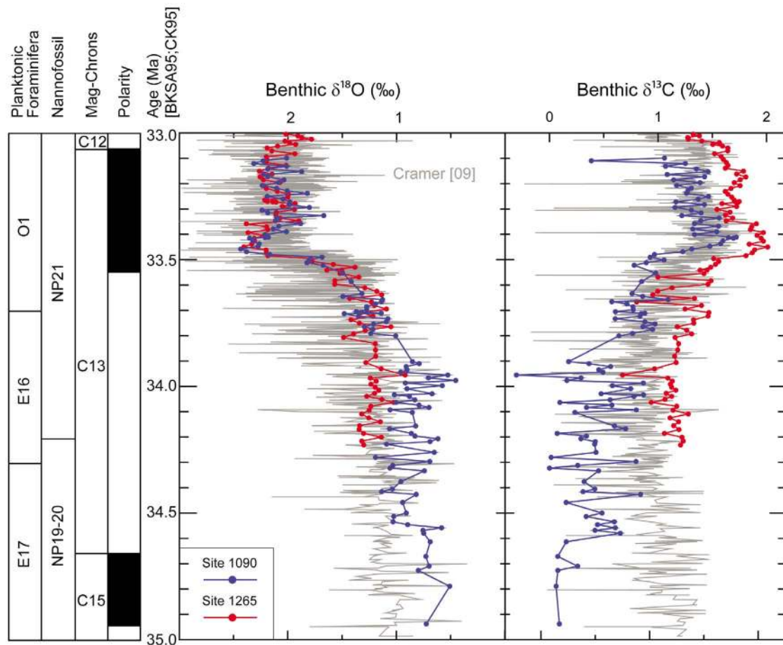
Figure 4. Benthic foraminiferal \delta^{18}\text{O} and \delta^{13}\text{C} isotope records across the Eocene-Oligocene transition from ODP Sites 1090 (blue circles; this work) and 1265 (red circles; this work) versus age in millions of years. The gray curve represents a recent compilation from Cramer et al. [2009]. Isotope values are reported relative to the VPDB (Vienna PeeDee belemnite) standard. The biostratigraphic age model follows Berggren et al. [1995], BKSA95; Cande and Kent [1995], CK95; and Berggren and Pearson [2005].
