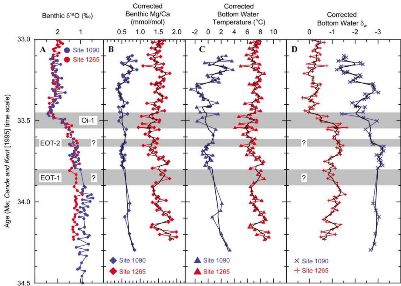
Figure 8. ODP Sites 1090 and 1265 benthic foraminiferal \delta^{18}\text{O} , corrected Mg/Ca, corrected bottom water temperature (BWT), and corrected seawater \delta^{18}\text{O} records versus age in millions of years. (a) Benthic foraminiferal ( Cibicidoides spp.) \delta^{18}\text{O} records from Sites 1090 (blue circles) and 1265 (red circles). Isotope values are reported relative to the VPDB (Vienna PeeDee belemnite) standard. (b) Sites 1090 (blue diamonds; Cibicidoides spp.) and 1265 (red diamonds; C. praemundulus ) benthic foraminiferal Mg/Ca ratios in mmol/mol corrected for changes in the deep water carbonate ion concentration associated with Oi-1 [Peck et al., 2010; Lear et al., 2010]; black lines show three-point running average. (c) Adjusted bottom water temperatures (BWT) corrected for changes in the carbonate ion concentration from Sites 1090 (blue triangles) and Site 1265 (red triangles) calculated from adjusted benthic foraminiferal Mg/Ca data in Figure 8b using the benthic foraminiferal calibration of Raitzsch et al. [2008] with the modern-day Mg/Ca seawater value (5.1 mmol/mol) and assuming Mg/Ca = 4.3 mmol/mol at 34 Ma; black lines display three-point running average. (d) Corrected bottom water \delta^{18}\text{O} ( \delta_w ) calculated from benthic foraminiferal \delta^{18}\text{O} data in Figure 8a and adjusted BWT in Figure 8c using the equation of Shackleton [1974]. Gray bars mark the EOT-1 (Eocene-Oligocene transition event 1), EOT-2 (Eocene-Oligocene transition event 2), and Oi-1 (Oligocene isotope event 1) events occurring at 33.8, 33.63, and 33.54 Ma, respectively [Miller et al., 1991, 2008; Lear et al., 2004; Coxall et al., 2005; Katz et al., 2008].
