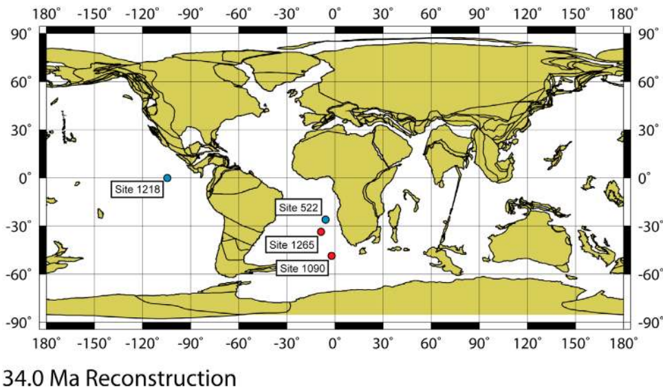
Figure 1. Paleogeographic reconstruction for 34 Ma showing the locations of Ocean Drilling Program (ODP) Sites 1090 and 1265 used in this study (red circles) and Deep Sea Drilling Project (DSDP) Site 522 and ODP Site 1218 (blue circles) from previous studies [Zachos et al. , 1996; Coxall et al. , 2005]. The map was created using the Ocean Drilling Stratigraphic Network ( http://www.odsnet.de/ ).
