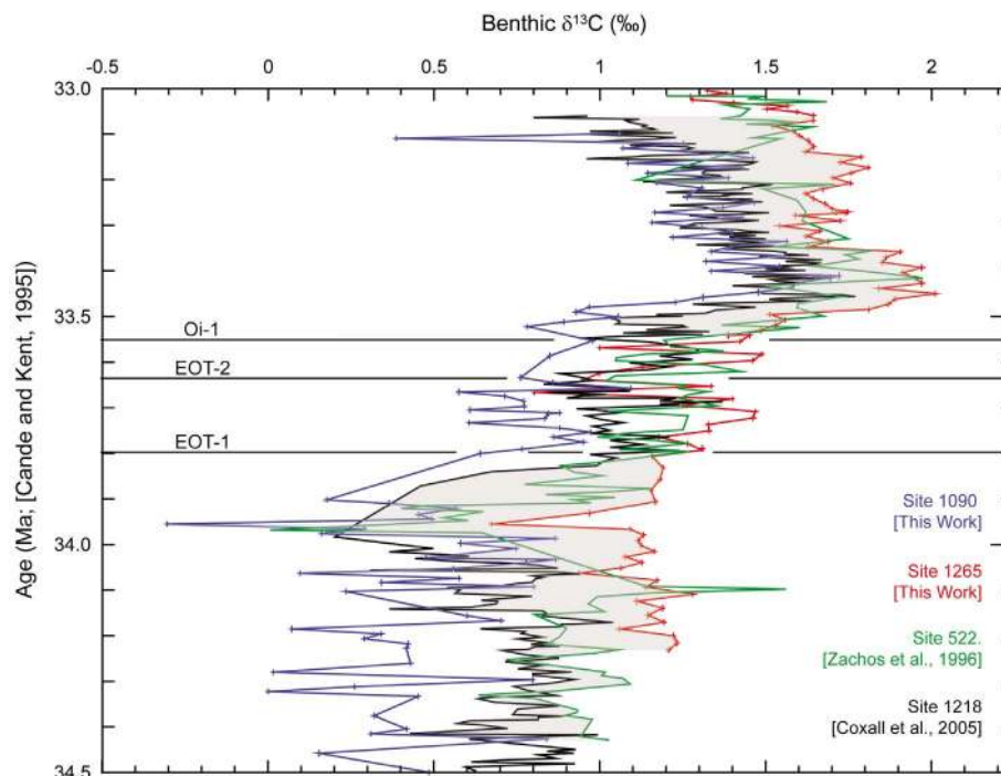
Figure 6. Summary of the latest Eocene to earliest Oligocene \delta^{13}\text{C} ratios for Cibicidoides from Southern Ocean ODP Site 1090, east Atlantic ODP Site 1265, east Atlantic DSDP Site 522 [Zachos et al. , 1996], and Pacific Ocean ODP Site 1218 [Coxall et al. , 2005]. Site 1090 represents the Southern Ocean end-member, with Site 1218 [Coxall et al. , 2005] serving as the Pacific end-member for deep water during the EOT. Gray shading illustrates the influence of a more nutrient-depleted water mass at Sites 1265 and 522 [Zachos et al. , 1996]. The \delta^{18}\text{O} and \delta^{13}\text{C} values are reported relative to the VPDB (Vienna PeeDee belemnite) standard. Black horizontal lines mark the EOT-1 (Eocene-Oligocene transition event 1), EOT-2 (Eocene-Oligocene transition event 2), and Oi-1 (Oligocene isotope event 1) events occurring at 33.8, 33.63, and 33.54 Ma, respectively [Miller et al. , 1991, 2008; Lear et al. , 2004; Coxall et al. , 2005; Katz et al. , 2008].
