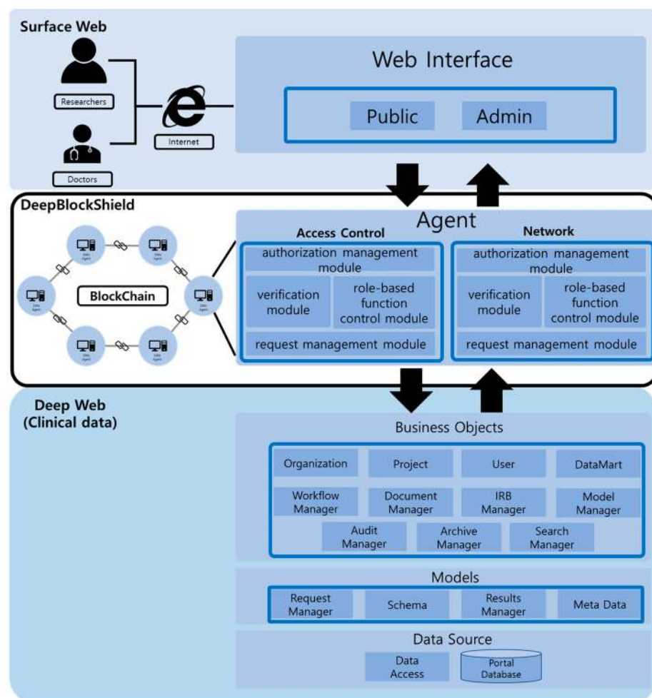
Figure 2. DeepBlockShield Overview.
