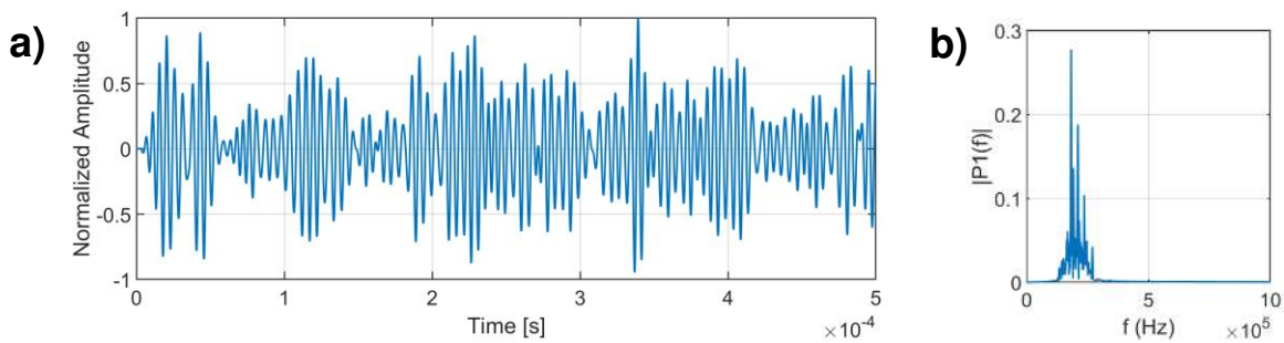
Figure 5a – b: Captured Lamb wave signal in time-domain (left) and its representation in frequency-domain (right)
