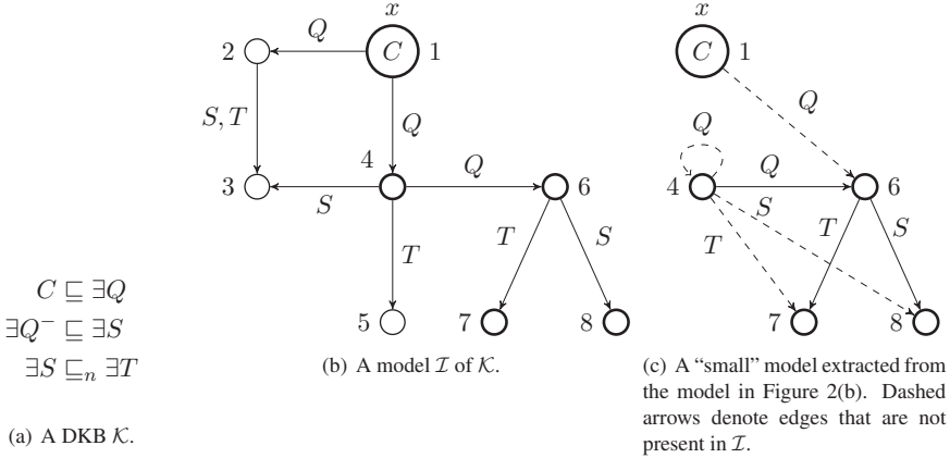
Figure 2: Illustrating Lemma 6.1.
