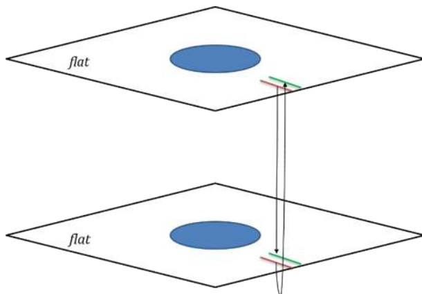
Figure 6. Replica trick without replica wormhole for n = 2 replicas.
