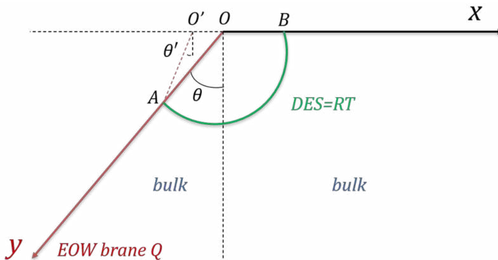
Figure 2. DES in original BCFT treated as the RT surface in BCFT'.
