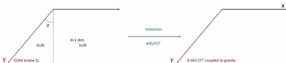
Figure 5. Effective description with Neumann boundary condition.
