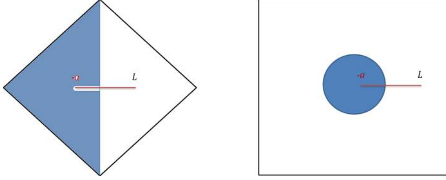
Figure 8. n -fold cover of effective boundary configuration in Lorentzian signature (left) and Euclidean signature (right).
