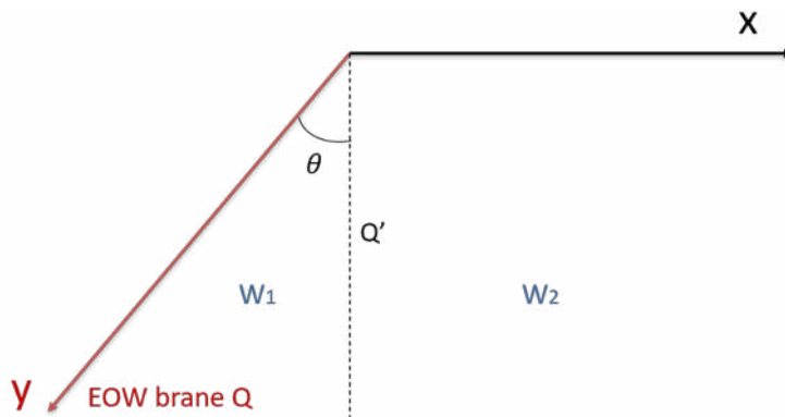
Figure 4. Bulk decomposition by inserting an imaginary boundary Q' .
