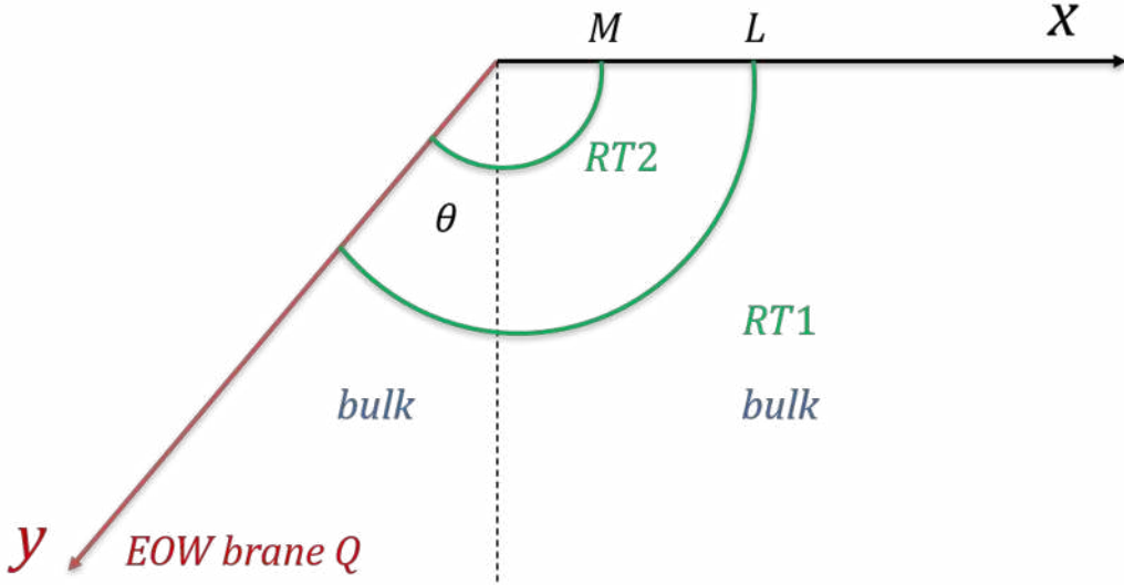
Figure 3. Defect extremal surface in the disconnected phase.
