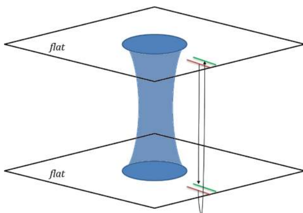
Figure 7. Replica wormhole that connects gravity region of the two copies.
