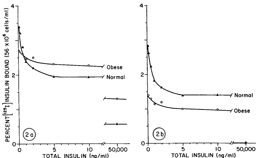
FIGURE 2 [^{125}\text{I}] insulin binding to lymphocytes from one obese and one normal subject. One normal thin volunteer and one obese patient were studied simultaneously under the same conditions. Blood was drawn, and the lymphocytes were isolated by centrifugation in a Ficoll-Hypaque gradient. [^{125}\text{I}] insulin (0.1 ng/ml) was incubated with lymphocytes ( 56 \times 10^6 /ml) in the absence of unlabeled insulin and in the presence of a range of concentrations of unlabeled insulin up to 50,000 ng/ml. After 90 min at 15^\circ\text{C} , duplicate aliquots of the incubation solutions were transferred to microfuge tubes and centrifuged. The supernates were aspirated and discarded; the cell pellet at the bottom of each tube was excised and the radioactivity counted. Each point is the mean of duplicates. In Fig. 2 a, total binding, expressed as the percentage of total radioactivity per milliliter that was bound to 56 \times 10^6 cells/ml, is plotted on the vertical axis as a function of the total insulin concentration. Nonspecific binding is the radioactivity bound to the cells in the presence of unlabeled insulin at 50,000 ng/ml. Specific binding is the difference between total binding and nonspecific binding. In Fig. 2 b, the same data are presented except that specific binding, rather than total binding, is plotted on the vertical axis. Although not shown in these graphs, points at insulin concentrations of 30, 100, and 1,000 ng/ml were also included in all experiments.
