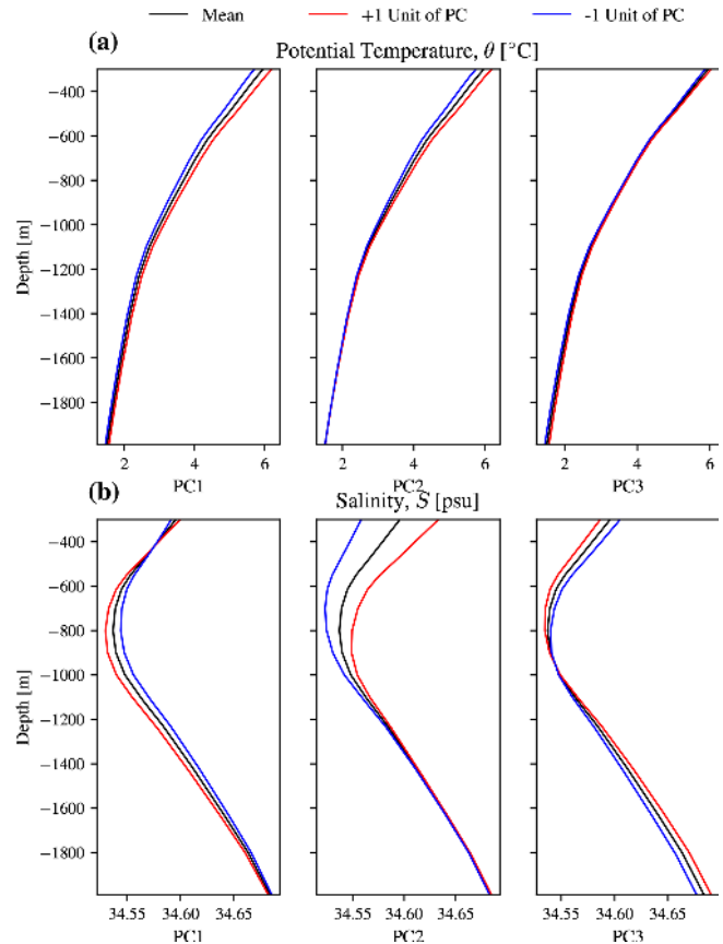
Figure B2. The temperature and salinity components of the three retained principal components that were used in this work. Specifically, they are PC1 (left column), PC2 (middle column), and PC3 (right column). Shown are the mean structures (black lines) with the effect of adding (red line) or removing (blue line) one unit of a principal component as a deviation from the mean profile, after Fig. 4 in Pauthenet et al. (2017). When compared to Fig. 1 we can see that PC1 corresponds to the hot–cold north–south contrast.
