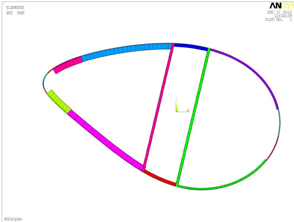
Figure 4: 6.9m span; TE reinforcement, foam, spar cap, some root reinforcement; circular/DU99-W-405 blend
