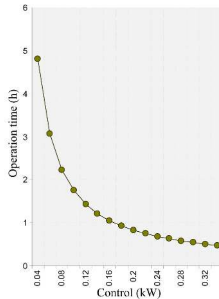
Fig. 13. Change of heating operation time from temperature depending on control
