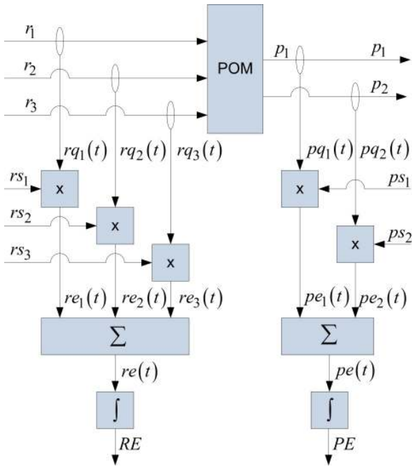
Fig. 3. Principle of product operation model formation: POM – product operation model
