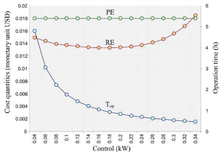
Fig. 14. Changes in the basic parameters of the simple operation model depending on control
