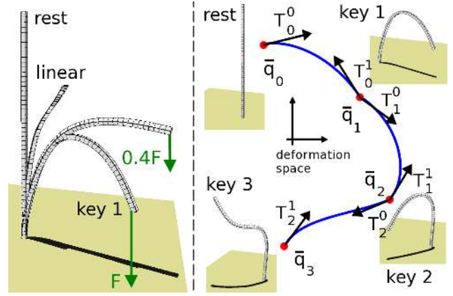
Figure 4: Our basis captures the natural deformations connecting the keyframes: Left: User sets a keyframe by pulling on the end of a beam (force F ), using an interactive static solver. The static equilibrium under an interpolated load ( \alpha = 0.4 ) is a natural shape, whereas a mere linear interpolation is severely distorted. Right: Three consecutive arcs on the keyframe deformation curve.
