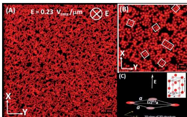
Fig. 4 (A) Image of a sample at \phi_{\text{eff}} = 0.85 and E = 0.23 \text{ V}_{\text{rms}} \mu\text{m}^{-1} applied along the Z-direction using a 3\times zoom. Objective: 63\times oil immersion. (B) Expanded sub-region highlighting small crystallites (squares in the X–Y plane) coexisting with voids. (C) Schematic representation of the BCT unit cell and its square base in the X–Y image plane.
