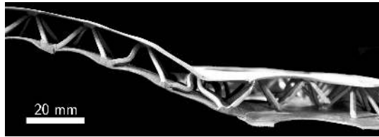
(b) detail of buckled truss members
