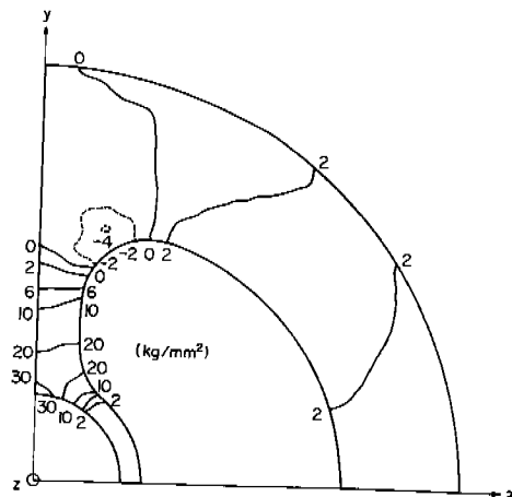
Fig.11 Contour plots of stress intensity of valve in y direction under free deformation.
