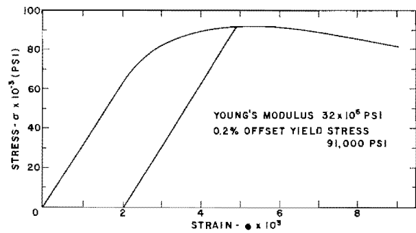
Fig. 3—Tensile stress-strain curve of a thin steel sheet
