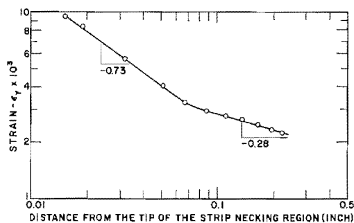
Fig. 5—Strain ahead of the strip necking region
