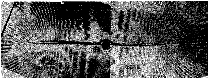
Fig. 1—Moiré pattern of a steel specimen: applied stress, 55 ksi; 0.2-percent-offset yield stress, 91 ksi; Young's modulus, 32 \times 10^6 psi; 0.012-in. thick; 6-in. wide; slot length, 1.0 in.; pitch of moiré grille, 1/13,400 in.
