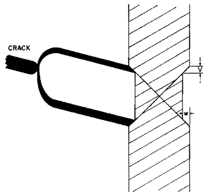
Fig. 7—Schematic diagram for necking zone ahead of a crack
