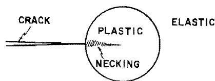
Fig. 6—Schematic diagram of the various regions of deformation around a crack
