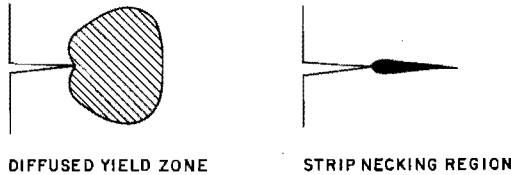
Fig. 2—Schematic diagrams of diffused yield zone and strip necking region
