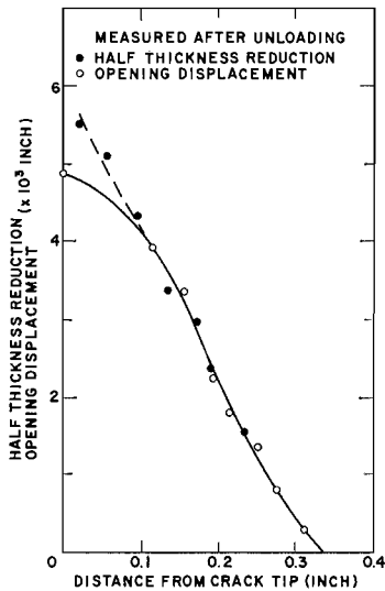
Fig. 8—Half-thickness reduction and opening displacement in the strip necking region of a steel specimen. \sigma , 62 ksi
