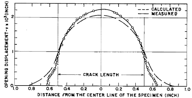
Fig. 4—Opening displacement along crack line: \sigma , 55 ksi; \sigma_Y , 91 ksi; E , 32 \times 10^6 psi; thickness, 0.012 in.; width, 6 in.; slot length, 1.0 in.
