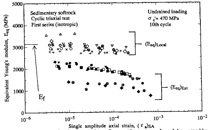
Fig. 18 Part of the results from the round-robin cyclic triaxial test program using sedimentary soft mudstone organized by JSSMFE; comparison of E_{eq} \sim \log(\epsilon_a)_{SA} relations obtained from eight tests (Fig. 3-16a of Toki et al., 1994).
