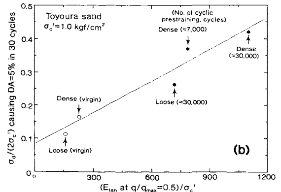
Fig. 56 Relationships between liquefaction strength and a) normalized maximum contractancy and b) normalized tangent Young's modulus E_{tan} at q/q_{max}=0.5 for virgin and cyclically prestrained Toyoura sand (Teachavorasinskun et al., 1994).
