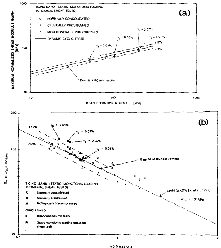
Fig. 39 Comparison of the maximum shear moduli G_{max} plotted against (a) mean pressure p of Ticino sand, and (b) void ratio of Ticino sand and Quiou sand for \sigma'_m = 100 kPa, obtained from several different testing methods (Lo Presti et al., 1993); For the resonant-column tests, the specimens were solid cylindrical (66 tests with 7.1 cm in D and 14 cm in H; Lo Presti, 1987, and four tests with 5 cm in D and 10 cm in H; Armandi, 1991). For 27 static ML torsional shear tests, he specimens were solid cylindrical (5 cm in D and 10 cm in H) at a shear strain rate of 0.002%/min. (Armandi, 1991, Lo Presti et al., 1993). For Quiou sand, the torsional resonant-column tests were five tests with 5 cm in D and 10 cm and three tests with 7.1 cm in OD, 5 cm in ID and 14.2 cm in H), and the static ML torsional shear tests were five tests (7.1 cm in OD, 5 cm in ID and 14.2 cm in H) (Lo Presti et al., 1993, Pallara, 1995).
