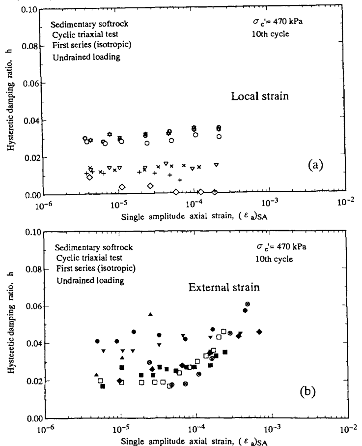
Fig. 19 Part of the results from the round-robin cyclic triaxial test program organized by JSSMFE using sedimentary soft mudstone; comparison of h \sim \log(\epsilon_a)_{SA} relations, corresponding to Fig. 18; a) local and b) external strain measurements (Fig. 3-17 of Toki et al., 1994).
