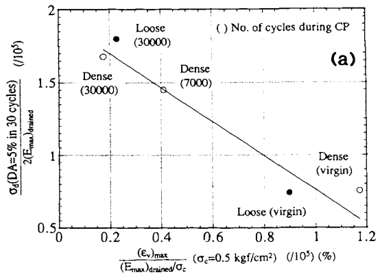
Fig. 55 Relationship between liquefaction strength and normalized maximum Young's modulus E_{max} for virgin and cyclically prestrained Toyoura sand (Teachavorasinskun et al., 1992, 1994).
