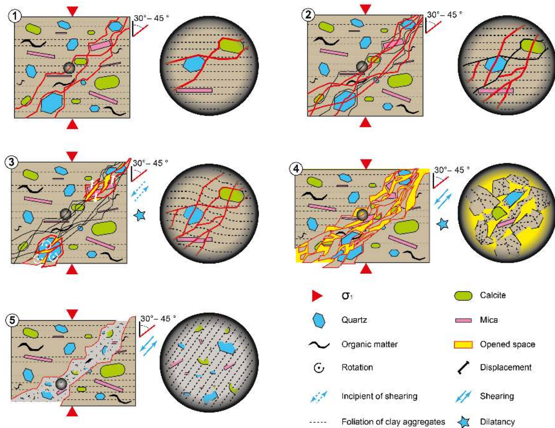
Figure 12. Conceptual model of microstructure development in triaxially deformed COX. (1) and (2) show microfracturing. In (1) intergranular microcracking initiating at non-clay minerals and clay minerals (NCM–CM) interfaces and propagating within CM. In (2) fragmentation of original fabric by transgranular and intragranular microfracturing of NCM. (3, 4) Cataclastic shearing with plasticity of phyllosilicates, macroscopic failure. In (3) incipient of shearing enhanced by plasticity of phyllosilicates at microfracture boundaries initiates cataclastic flow of original fabric's fragments. In (4) ongoing shearing drives cataclastic flow, and reworking of CM in original fabric's fragments. (5) Resealing of the damage zone by shear and pore collapse, evolution of clay gouge. See text for details. CM: clay matrix; NCM: non-clay minerals.
