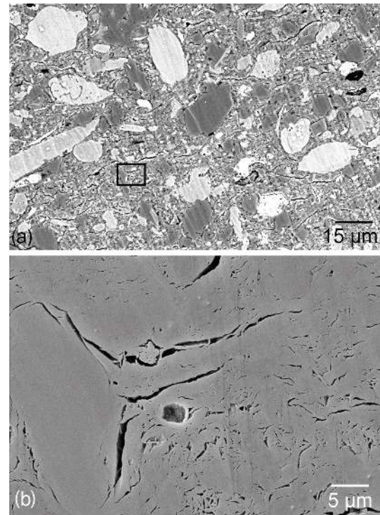
Figure 4. (a) BSE–SEM micrograph of the typical mineral fabric in undeformed COX. (b) SE2 SEM micrograph of a detail indicated by the black box in (a) showing the typical pore fabric in undeformed COX. In both micrographs, the bedding is horizontal.
