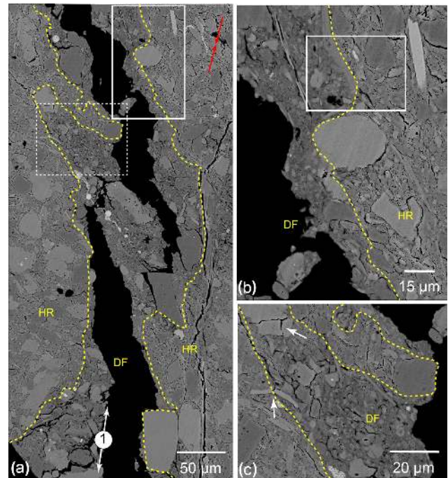
Figure 9. Microstructures of ROI-1 in sample COX-10MPa. (a–c) The damaged fabric (DF) within the main fracture (1) is made of fragments of non-clay minerals derived from the dense, tight clay matrix. (a) The large open fracture in the middle of the main fracture (black) is interpreted to develop after the experiment by unloading and/or drying (see Sect. 5.1 for details). In (a) the white box in dashed lines refers to (c), whereas the one in solid lines refers to (b). (b) Details of difference in mineral fabric between DF and the host rock (HR). The white box refers to Fig. 10. (c) Some grains within the damaged fabric, but close to the boundary between the damaged fabric and the host rock, show transgranular fracturing (white arrows). In all micrographs, the orientation of the principal stress ( \sigma_1 ) is indicated by red arrows. The bedding is perpendicular to \sigma_1 . The dashed yellow lines indicate the boundaries between DF and HR.
