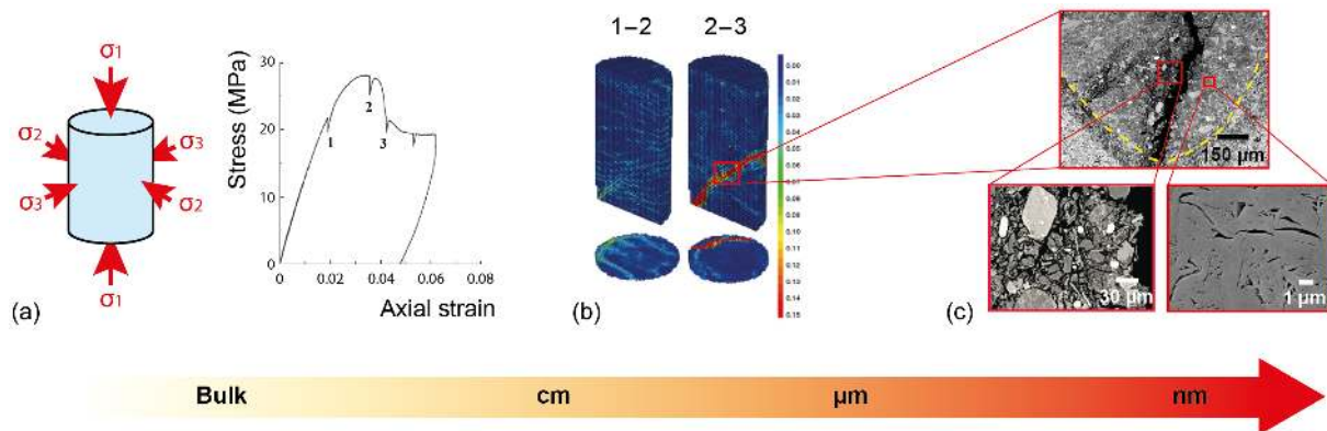
Figure 1. Drawing of the experimental concept used for the investigation of experimentally deformed fine-grained mudrocks from bulk scale to nanometre scale. The example is based on (a) a triaxial deformation test (10 MPa confining pressure) performed on a cylindrical Callovo–Oxfordian Clay, (b) volumetric DIC on X-ray microtomography images to follow displacement fields (after Lenoir et al., 2007), and (c) SEM imaging on high-quality cross sections prepared by BIB. (a) Steps when X-ray microtomography images were acquired are indicated by 1, 2 and 3. (b) Deformation increments between steps 1 and 2 and steps 2 and 3 are indicated by 1–2 and 2–3 respectively.
