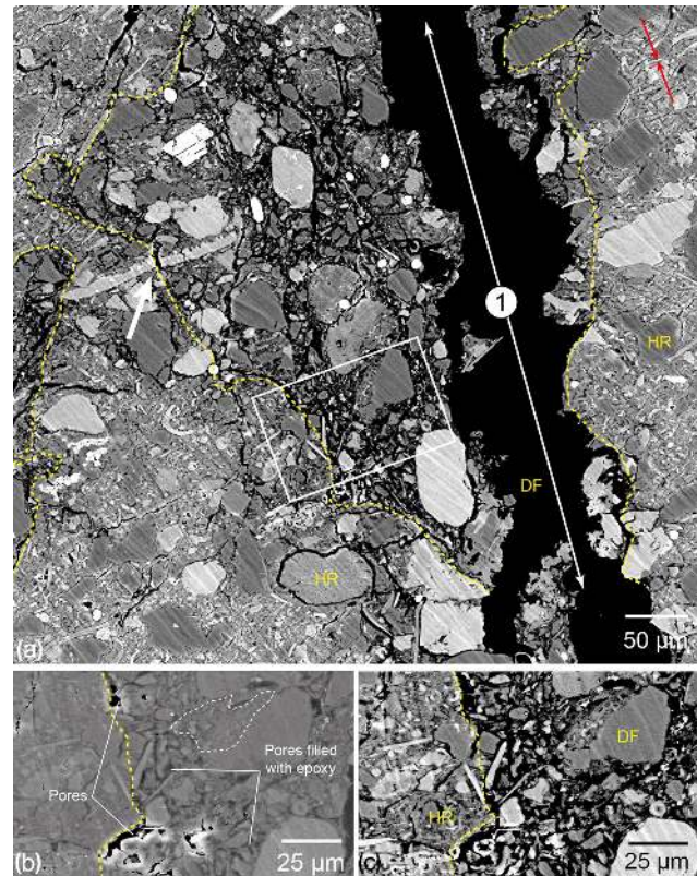
Figure 11. Detailed microstructures at ROI-2 in sample COX-10MPa. (a–c) The damaged fabric (DF) within the main synthetic fracture (indicated by number 1) is made of fragments of non-clay minerals and clay matrix derived from the host rock (HR). (a) Some grains within the damaged fabric, but close to the boundary between the damaged fabric and the host rock, show transgranular fracturing (white arrow). The white box refers to Fig. 11a and b. Detailed observations in (b) and c (SE2 SEM and BSE-SEM micrographs of the same sub-area, respectively) show that parts of the damaged fabric display (1) porous island, where pores are between the fragments of non-clay and clay matrix, whereas other parts display (2) low porous islands made of fragments of non-clay minerals embedded in a dense, tight clay matrix (within the region bounded by the dashed white line). Pores within the porous island can either be filled with epoxy (in deep black pixel values) or not. The orientation of the principal stress ( \sigma_1 ) is indicated by red arrows. The bedding is perpendicular to \sigma_1 . The dashed yellow lines indicate the boundaries between the damaged fabric and the host rock.
