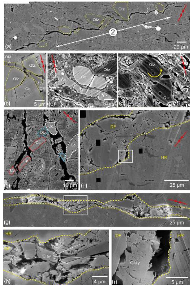
Figure 7. Detailed microstructures in sample COX-2MPa. (a) A fracture running parallel to the antithetic fractures and at the interfaces between non-clay mineral and clay matrix. In (b) intragranular fractures are in calcite grain (Cc.) and transgranular fractures are in organic matter (OM), whereas in (c) transgranular fractures are in Cc. at impingement with quartz grain (Qtz.). (d) A broken quartz grain showing evidence for rotation of its broken fragments. (e) Incipient of flow of broken non-clay minerals within the antithetic fractures indicated by red (Cc.), blue (Qtz.) and white (Cc.) dashed lines. (f) and (g) show parts of antithetic fractures displaying thick damaged fabrics made of broken grains and clay matrix fragments. (h) Details of the white box indicated in (g). (i) Details of the white box indicated in (f), showing the denser and deformed fabric of a part of the clay matrix squeezed between a quartz grain located in the damaged fabric and the boundary with the host rock. In (f)–(i), the damaged fabric is related to a higher porosity in comparison to the host rock. In all micrographs, the orientation of the principal stress ( \sigma_1 ) is indicated by red arrows. The bedding is perpendicular to \sigma_1 . Dashed yellow lines indicate the boundaries between the damaged fabric (DF) and the host rock (HR) and also some grain boundaries in (a). Black squares in (f) are missing pictures.
