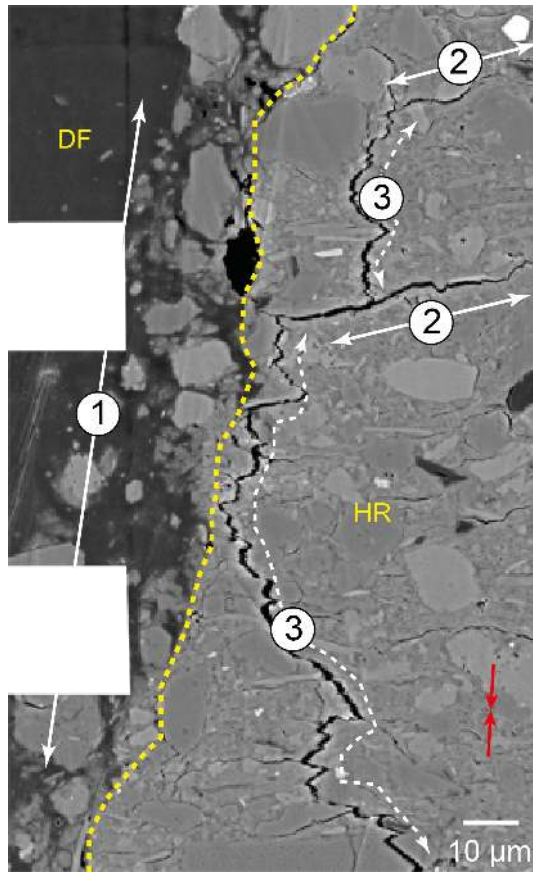
Figure 8. Detailed microstructure close the main fracture (indicated by number 1) in sample COX-2MPa. The main fracture displays internal damaged fabric made of fragments of broken non-clay minerals and clay matrix. Close to the main synthetic fracture, the host rock displays jagged joints subparallel to the main synthetic fracture (indicated by number 3) starting and ending at the antithetic fracture (indicated by number 2). In all micrographs, the orientation of the principal stress ( \sigma_1 ) is indicated by red arrows. The bedding is perpendicular to \sigma_1 . The dashed yellow line indicates the boundary between the damaged fabric (DF) and the host rock (HR).
