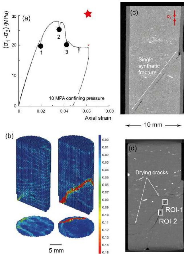
Figure 3. Results of deformation test done on sample COX-10MPa. (a) Deviator stress vs. axial strain response. The red star indicates the state of sample when BIB–SEM microstructural analyses are done. (b) Incremental maximum shear strain fields for deformation increments 1–2 and 2–3 indicated in (a) interpreted after DIC. (c) Shows the X-ray radiography of the sample taken directly at the end of the deformation test, whereas (d) shows the X-ray radiography of the same sample but taken about 10 years after the end of the deformation: drying cracks developed following the bedding, and the aperture of the single shear fracture became larger. (d) Also indicates that two ROI were analysed, both around the single synthetic shear fracture. In (c) and (d) the bedding is perpendicular to the principal stress \sigma_1 indicated in (c). Performed according to Lenoir et al. (2007).
