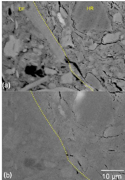
Figure 10. Details of Fig. 9b. Microstructures (ROI-1_COX-10MPa) showing details of porosity in BSE-SEM micrograph (a) and SE2 SEM micrograph (b). At the resolution of the SEM micrograph, the damaged fabric appears to be very low porous in comparison to the host rock. The dashed yellow line indicates the boundary between the damaged fabric (DF) and the host rock (HR).
