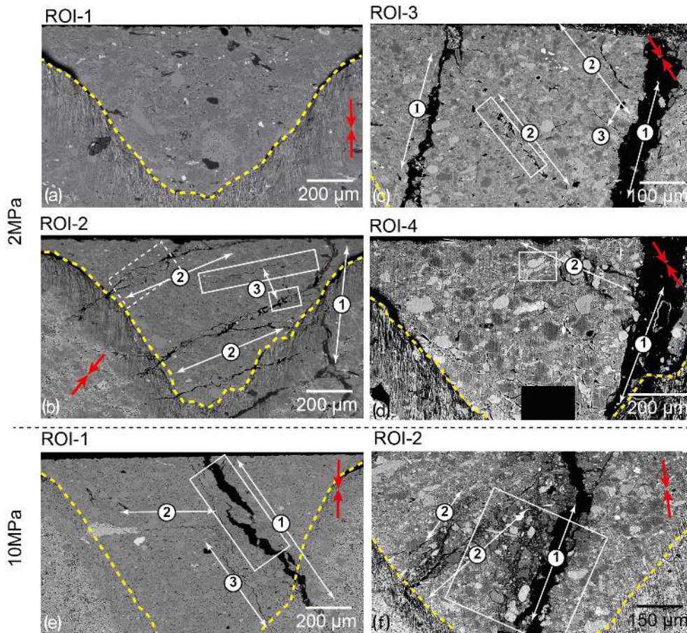
Figure 5. BSE-SEM micrographs of the BIB cross section overviews of COX-2MPa (a–d) and COX-10MPa (e–f) at differently strained areas (ROI) highlighted from DIC analysis in Figs. 2 and 3. Highly strained ROI (b–f) display damaged microstructures where three different types of fracture are identified: (1) the main synthetic fracture, (2) antithetic fractures oriented about 60^\circ to the main fracture and (3) joints subparallel to the main synthetic fracture. These fractures are respectively indicated by numbers 1, 2 and 3 in the figure. In (b) the white box in dashed lines refers to Fig. 7f; the upper white box in solid lines refers to Fig. 7a and the lower white box in solid lines refers to Fig. 7e. In (c) the white box in solid lines refers to Fig. 7g. In (d) the white box in solid lines refers to Fig. 7c. In (e) the white box in solid lines refers to Fig. 9. In (f) the white box in solid lines refers to Fig. 11. In all micrographs, the orientation of the principal stress ( \sigma_1 ) is indicated by red arrows. The bedding is perpendicular to \sigma_1 . Dashed yellow lines indicate the boundaries of the BIB-polished areas.
