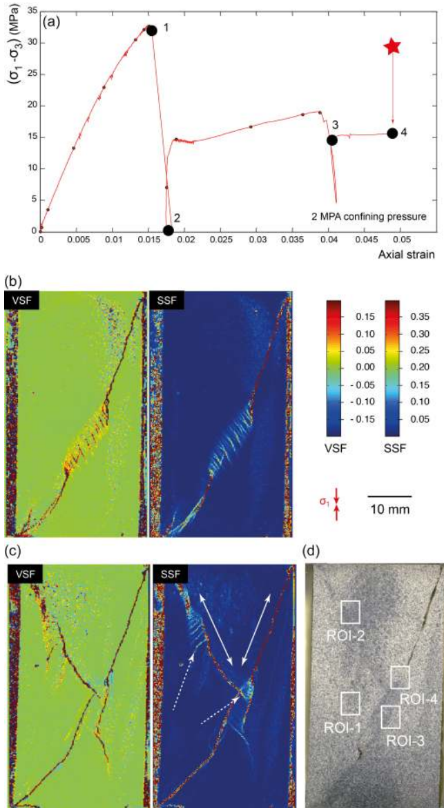
Figure 2. Results of deformation test done on sample COX-2MPa. (a) Deviator stress vs. axial strain response. The red star indicates the state of the sample when BIB–SEM microstructural analyses are done. (b, c) Incremental volumetric strain fields (VSF) and maximum shear strain fields (SSF) for deformation increments 1–2 (b) and 3–4 (c) indicated in (a) after DIC. Arrows with solid lines indicate the set of two conjugated synthetic fractures, whereas the arrows with dashed lines show antithetic fractures oblique to the conjugated fractures. (d) Selection of differently strained areas (region of interest (ROI)) highlighted from DIC analysis for BIB–SEM microstructural analyses. Four ROI were analysed: three at conjugate synthetic fractures in areas with a different amount of diffuse strain and antithetic fractures (ROI-2, ROI-3 and ROI-4) and one in a region without measurable strain (ROI-1). The bedding is perpendicular to the mean principal stress \sigma_1 . Performed according to Bésuelle et al. (2011).
