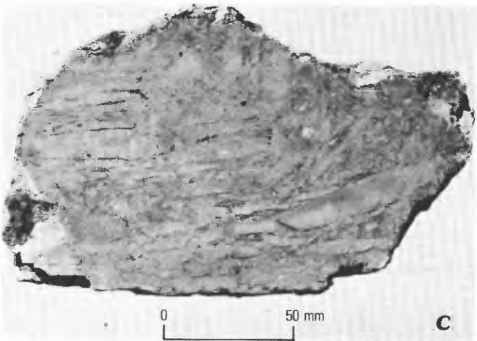
FIGURE 14.—Specimens of rocks from bud on dike segment 19. A , Heterobreccia. B , Fractured Mancos Shale from northernmost part of bud; fractures parallel contact with minette. C , Monobreccia from northernmost part of bud. Note brecciation and internal rotation and displacement of shale fragments.
