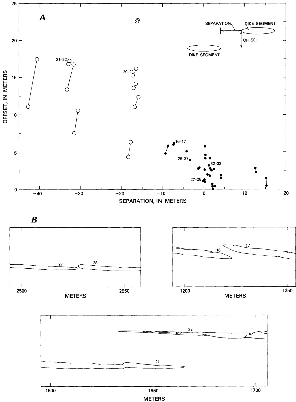
FIGURE 10.—Offset and separation relations for segments of northeastern dike. A , Offset as a function of separation (or overlap) for adjacent segments. Offset and separations are measured using strikes of adjacent segments as reference lines, and the two data points are connected by lines. Closed circles denote adjacent segments with less than 10 m of offset or separations; open circles, more than 10 m of offset or separation. Those segment pairs referred to in text are labeled. B , Typical forms of segment ends with different offset and separation. Numbers refer to dike segments in plate 1.
