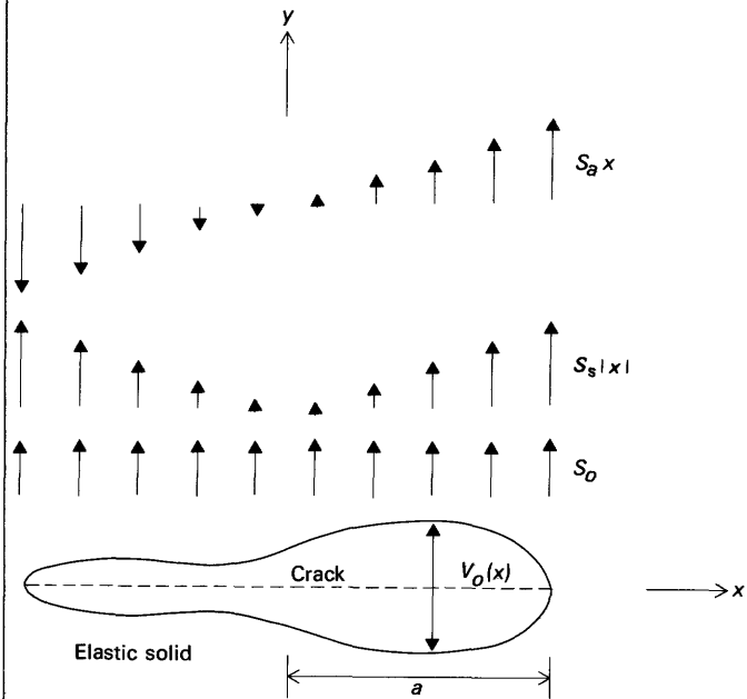
FIGURE 27.—Geometry and parameters of model used to calculate cross-sectional form of a crack in an elastic medium subjected to uniform normal stress ( S_0 ), symmetrical linear stress gradient ( S_s|x| ), and asymmetric linear stress gradient ( S_a x ). Dilation is given by 2v_0(x) ; a is half-width of crack.
