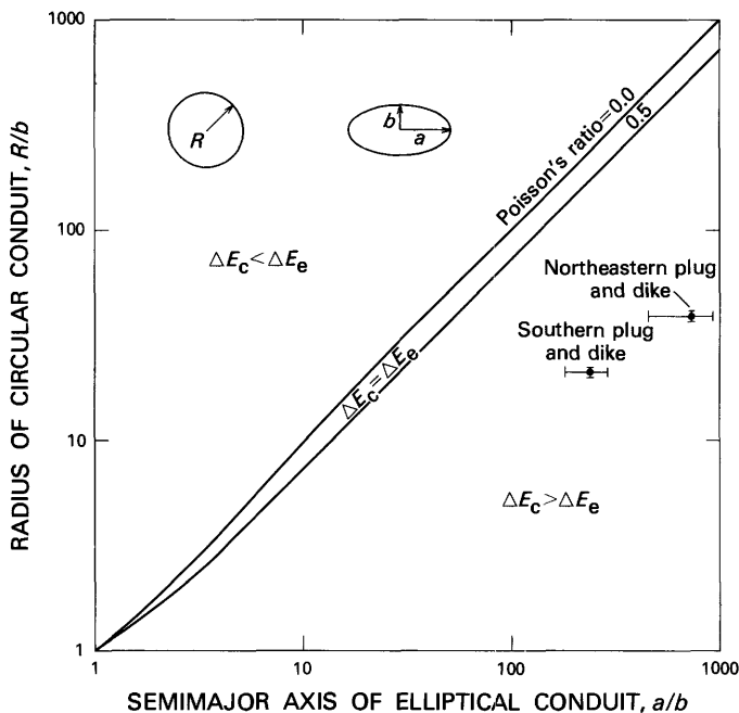
FIGURE 20.—Radius R of circular conduit as a function of semimajor axis a of elliptical conduit, both normalized by semimajor axis b of elliptical conduit. Two curves represent limits on possible range of Poisson's ratio and divide graph area into two fields in which work \Delta E_c done on elastic host rock during emplacement of given volume of magma in a circular conduit is either greater or less than work \Delta E_e done in elliptical conduit. Two data points with error bars are for spatially associated plugs and dikes near Ship Rock.
