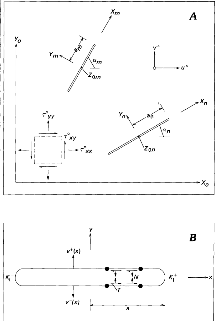
FIGURE 22.—Geometry and parameters of model used to calculate dilation and propagation of multiple interacting cracks by method of successive approximations. A, Parameters for cracks include center z_0 relative to global coordinates (x_0, y_0) , half-width a , angle \alpha , and local coordinates (x, y) . Each parameter is identified with a particular crack by an appropriate subscript. Stresses denoted by \sigma , and displacement by (u, v) ; positive directions indicated by arrows. B, Normal and tangential stresses N and T , respectively, acting uniformly over two opposing intervals of crack wall (area between dots); dilation is given by difference v^+(x) - v^-(x) . K_I^+ and K_I^- are mode I stress-intensity factors at x = \pm a , where a is half-width of crack.
