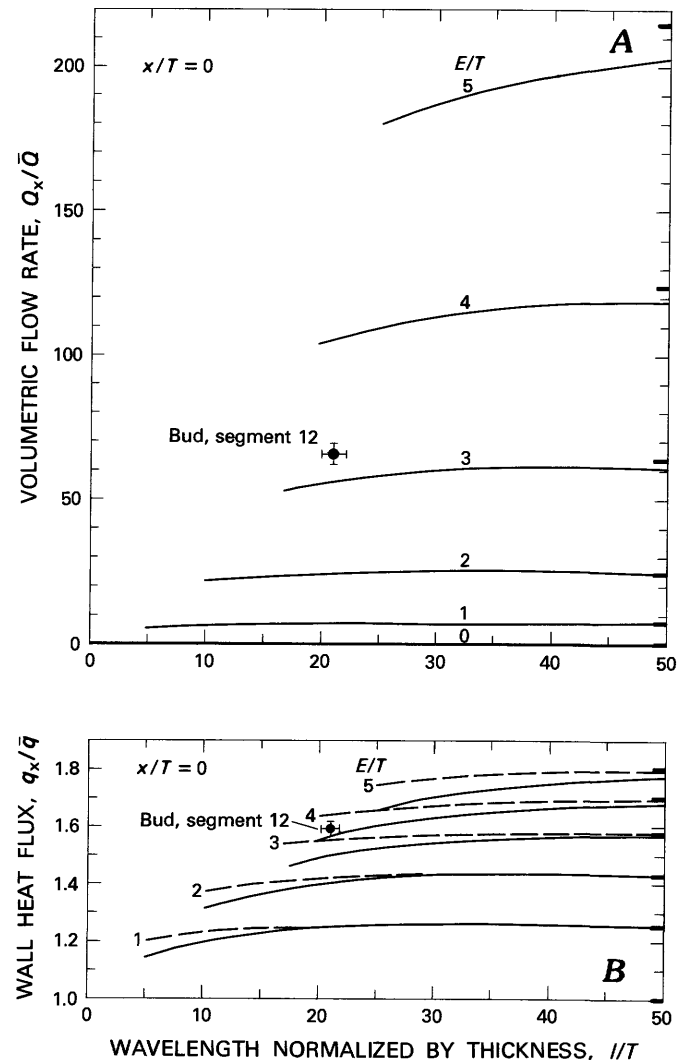
FIGURE 35.—Local volumetric flow rate (A) and wall heat flux (B) as functions of normalized wavelength at thickest parts of conduits ( x/T=0 ) illustrated in figure 33A. Local volumetric flow rate Q_x and wall heat flux q_x are normalized by those for a conduit of unit thickness T . Dashed curves show heat flux from straight wall of conduit, and solid curves that from curved wall. Solid bars on vertical axes show local flow rate and heat flux for a conduit of uniform thickness ( E/T=1 ). Discharge of magma from thickest part of bud on segment 12 was probably about 60 times that in adjacent nonbrecciated parts of segment. Rate of heat loss, however, was probably less than 1.6 times greater than in narrower part of segment.
