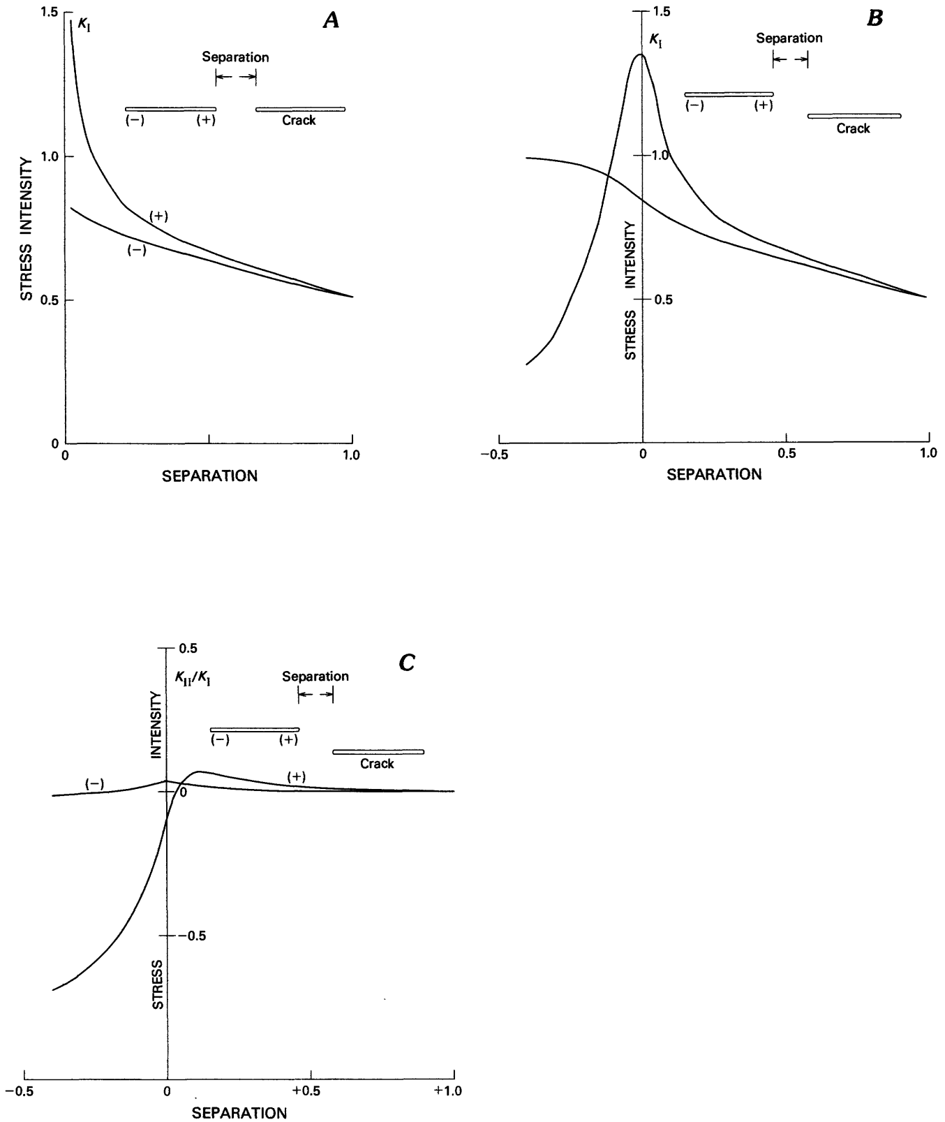
FIGURE 24.—Stress-intensity factors as a function of separation of pairs of collinear and offset cracks subjected to unit pressure (see fig. 23). Distal ends are fixed at x=+1 , and offset is 0.1. A, Mode I stress-intensity factor K_I as a function of separation of adjacent ends of pairs of collinear cracks. B, Mode I stress-intensity factor K_I as a function of separation of adjacent ends of pairs of offset pressurized cracks. C, Ratio of mode II to mode I stress-intensity factors K_{II}/K_I as a function of separation of adjacent ends.
