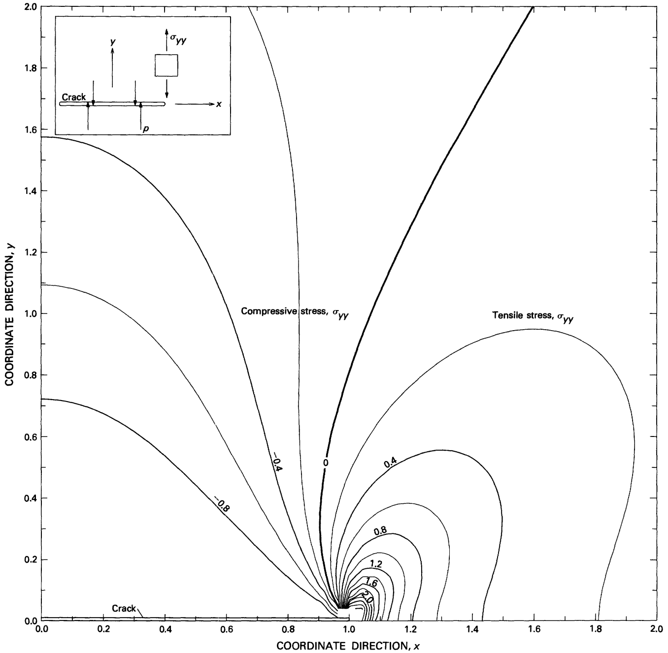
FIGURE 21.—Contours of stress component acting normal to pressurized crack, plotted in quadrant adjacent to crack; contours represent various ratios of stress \sigma_{yy} to driving pressure p . Contours are characterized by regions of compressive stress at side of crack and regions of tensile stress ahead of crack. Tensile stress increases to infinity at end of crack.
