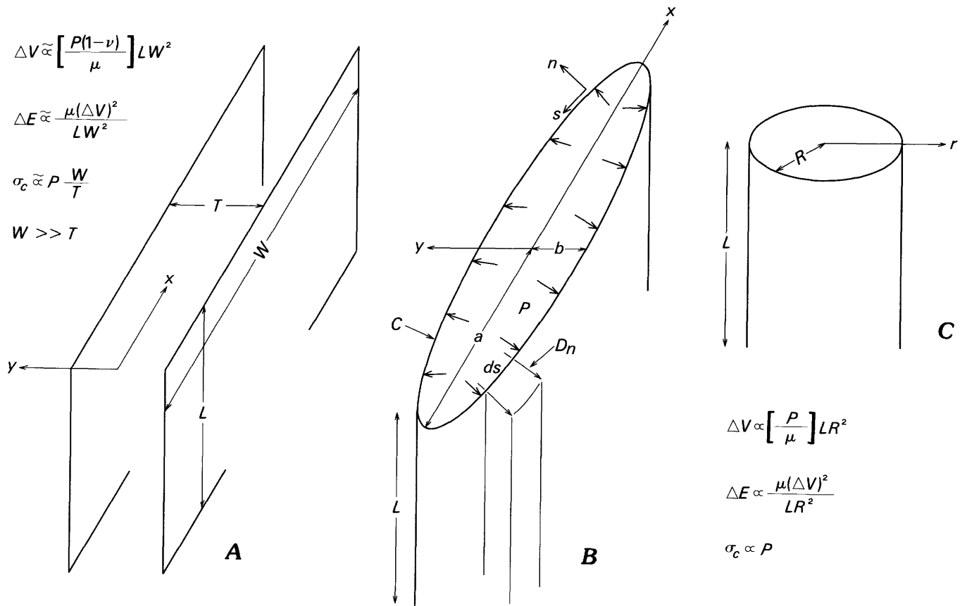
FIGURE 19.—Geometry and parameters of model used to calculate elastic deformation around idealized conduits, showing end members in spectrum of elliptical forms. A, Tabular conduit of thickness T , width W , and length L . B, Elliptical conduit with semimajor and semiminor axes a and b , respectively; C , contour of conduit wall; s and n , arc parameters defining position parallel and normal to C , respectively; ds , differential arc length along C ; D_n , component of displacement normal to wall; C, Circular conduit of radius R ; r , coordinate radial to conduit; \Delta V , volume change; P , pressure; \nu , Poisson's ratio; \mu , elastic shear modulus; \Delta E , work done on host rock; \sigma_c , component of normal stress acting parallel to wall. Coordinate directions are x , y , and z for tabular and elliptical conduits; r and z , for circular.
