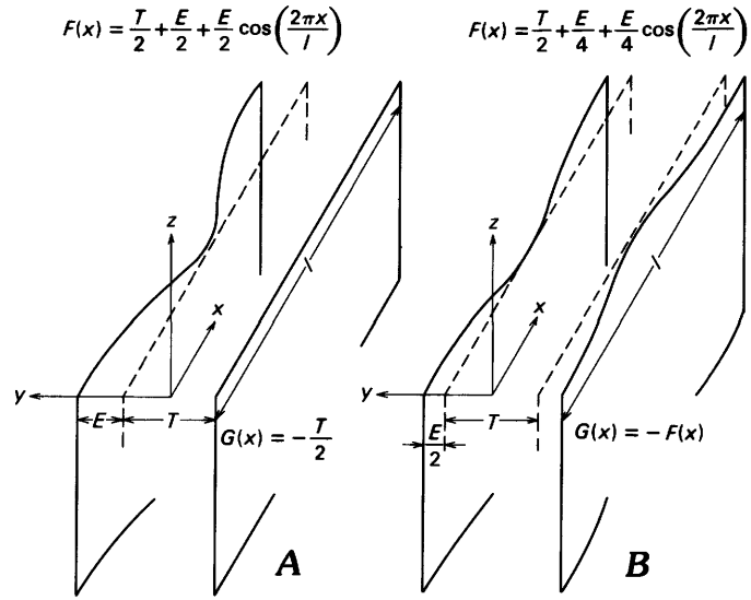
FIGURE 33.—Geometry and parameters of model used to calculate magma-flow and heat-loss rates in conduits of varying thickness. T , conduit thickness where not thickened; x , y , and z , coordinate directions. Limiting cases are that one wall (A) or both walls (B) vary sinusoidally according to functions y=F(x) and y=G(x) . Wavelength and total amount of thickening of sinusoidal curves are given by l and E , respectively.
