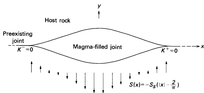
FIGURE 28.—Cross-sectional form of a crack subjected to a uniform linearly varying symmetrical stress distribution. Dilation is shown greatly exaggerated relative to width. This condition on driving pressure results in zero stress intensity ( K_I ) at crack ends and therefore is appropriate for magma pressurizing a pre-existing joint.
