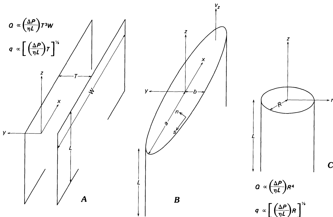
FIGURE 30.—Geometry and parameters of model for magma flow. A, Tabular conduit of thickness T , width W , and height L . B, Elliptical conduit with semimajor and semiminor axes a and b , respectively, and wall coordinate (s, n) defining distance along and normal to wall. C, Circular conduit of radius R . v , flow velocity; Q , volumetric flow rate; q_x , rate of heat loss at any position x along walls; \eta , viscosity; \Delta P/L , driving-pressure gradient. Flows in tabular and circular conduits are special cases of flow in an elliptical conduit (B); for an infinitely long dike (A), a = \infty and b = T/2 ; and for a plug (C), a = b = R . Coordinate directions x, y , and z are used for tabular and elliptical conduits; r and z , for circular conduit.
