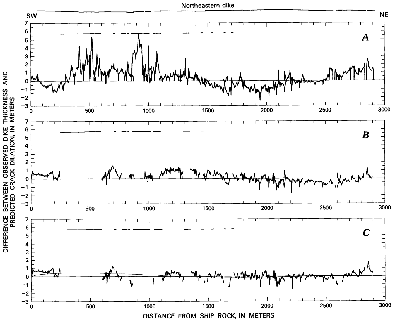
FIGURE 26.—Residuals between observed dike thickness and predicted crack dilation as a function of distance from Ship Rock; plots A, B, and C correspond to those in figure 25.
