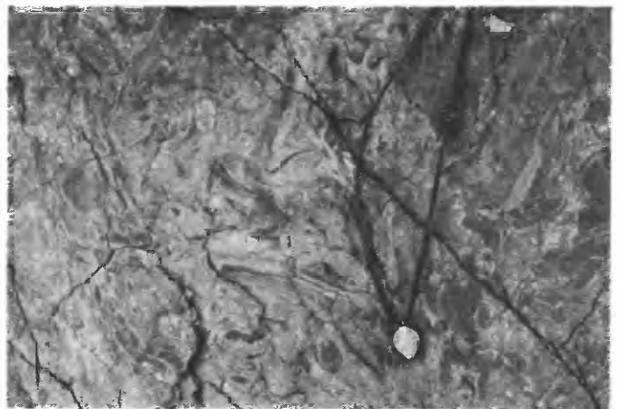
FIGURE 16.—Heterobreccia from northwestern plug, composed of fragments of siltstone, shale, and minette in a groundmass of finely comminuted sedimentary and igneous material. Streaky layering between dark stringers, and clasts of minette and intermixed light sandy material, suggest irregular flow banding.
