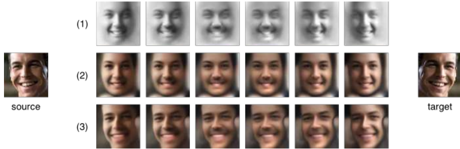
Fig. 10. Lighting interpolation with Intrinsic-DAE. With latent representations learned in an unsupervised manner for shading, albedo, and deformation, the DAE allows us to simulate smooth transitions of the lighting direction. In this example, we interpolate the latent representation of the shading from source (lit from the left) to target (mirrored source, hence lit from the right). The network generates smooth lighting transitions, without explicitly learning geometry, as shown in shading (1) and texture (2). Together with the learned deformation of the source image, DAE enables the relighting of the face in its original pose (3).
