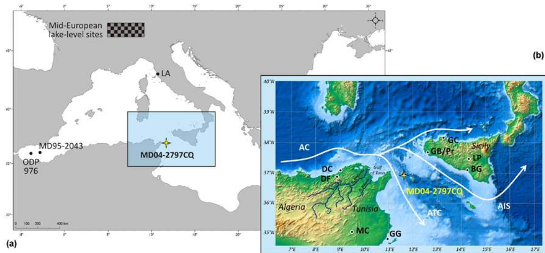
Fig. 1. Location of the studied core MD04-2797CQ and of other Mediterranean records mentioned in the text. (a) Large map: LA: Lake Accessa (Magny et al., 2007a; Finsinger et al., 2010), MD95-2043 (Fletcher and Sánchez Goñi, 2008), ODP site 976 (Combourieu-Nebout et al., 2009). Medjerda and Miliane river systems are indicated in dark blue. The mean sea surface circulation is represented by white arrows (AC: Algerian Current, ATC: Atlantic Tunisian Current, AIS: Atlantic Ionian Stream). (b) Inset map: sites from the southern Central Mediterranean. DF: Dar Fatma (Ben Tiba and Reille, 1982), MH: Majen Ben M’Hida (Stambouli-Essassi et al., 2007), GB/Pr: Gorgo Basso and Lake Preola (Tinner et al., 2009; Magny et al., 2011b), LP: Lake Pergusa (Sadori and Narcisi, 2001), BG: Biviera di Gela (Noti et al., 2009), MC: La Mine Cave (Genty et al., 2006), GC: Grotta di Carburangeli (Frisia et al., 2006).
