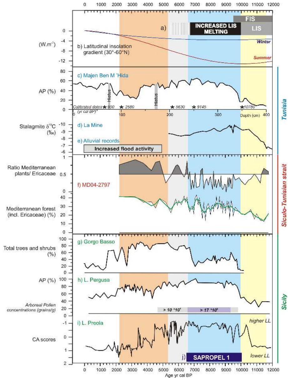
Fig. 6. Comparison of the pollen data from core MD04-2797CQ with other records from southern Central Mediterranean and with insolation and ice sheet forcings. Forcings – (a) Early Holocene ice sheet deglaciation: disappearance of the Fennoscandian Ice Sheet (FIS) at 9.5 kyr cal BP (Lundqvist and Saarnisto, 1995) and enhanced Laurentide Ice Sheet (LIS) retreat between 10 and 6.8 kyr cal BP with only small ice caps remaining up to 5.5 ka (Carlson et al., 2008); (b) Summer (JJA) and winter (DJF) latitudinal insolation gradient calculated from insolation values at 60° and 30° N (Berger and Loutre, 1991); Tunisia – (c) Majen Ben M’Hida peat pollen sequence: digitalized data versus depth (Stambouli-Essassi et al., 2007), asterisks: original dated levels (65 cm: 985 ± 30 yr BP; 100 cm: 2500 ± 50 yr BP; 205 cm: 4894 ± 40 yr BP; 250 cm: 8190 ± 50 yr BP; 350 cm: 9480 ± 100 yr BP) and calibrated ages using Calib 6.11 (903 (873–959); 2578 (2365–2740); 5629 (5585–5716); 9144 (9014–9287); 10 782 (10504–11143) yr cal BP); (d) δ 13 C speleothem record from the La Mine Cave (Genty et al., 2006); (e) Shaded bar representing the increased fluvial dynamics since 5 ka with recurrent floods associated to drier conditions, based on alluvial sequences from arid to semi-arid Central and North Tunisian floodplains (Zielhofer and Faust, 2008); Siculo-Tunisian Strait – (f) MD04-2797CQ pollen data: total tree and shrub percentages including Ericaceae with smoothing cubic spline (bold green line) and ratio of Mediterranean plants to Ericaceae; Sicily – (g) Total trees and shrubs percentages from Gorgo Basso pollen sequence (Tinner et al., 2009); (h) Arboreal pollen percentages and concentrations from Lake Pergusa sequence (Sadori and Narcisi, 2001; Sadori et al., 2011); (i) Relative changes in lake level (LL) from Lake Preola (Magny et al., 2011b); (j) Interval corresponding to Sapropel 1 after Mercone et al. (2000). The colored vertical bars represent the successive intervals as described in the text: yellow for the dry interval at the beginning of the early Holocene, blue for the wet early Holocene phase, grey for the mid-Holocene transitional interval and orange for the mid- to late Holocene phase of increasing dryness.
