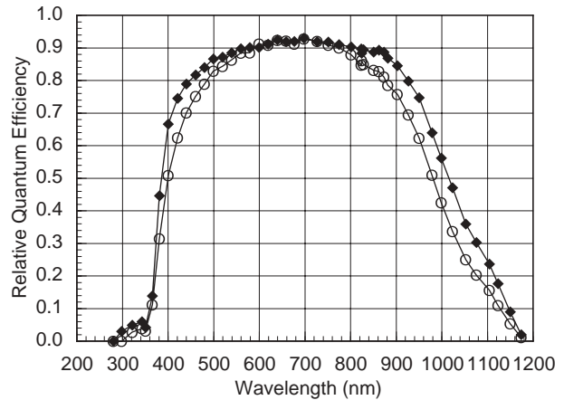
Fig. 2. Relative quantum efficiency for two individual cells from the Single #2 control and XR-260 modules, normalized to the unexposed ( \blacklozenge ) and exposed ( \circ ) I_{\text{sc}} values of the XR-260 module (see text).
