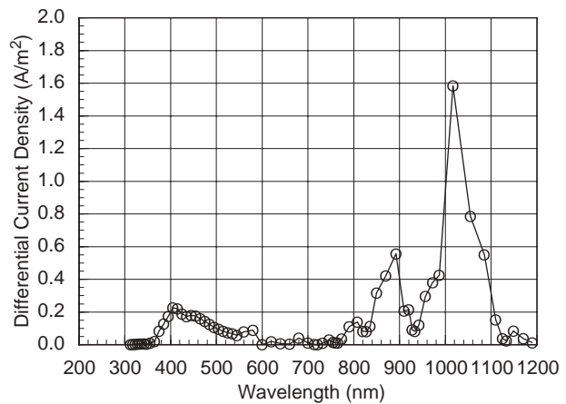
Fig. 3. The difference between the two QE curves in Fig. 2, weighted by the standard global reference spectrum, as a function of wavelength. The total I_{\text{sc}} loss in the exposed cell was -6.7%; the short wavelength loss was -1.8% and the long wavelength loss was -4.9%. Note that the total loss amount includes the rapid initial light-induced degradation of -3.8%.
