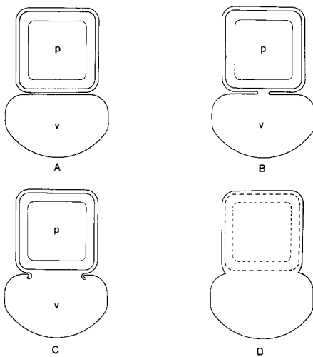
Fig. 24A—D. Schematic drawing of the migration of an intact peroxisome into a central vacuole (or autophagic vacuole) as a result of fusion of the electron-dense membranes with the vacuolar membrane
