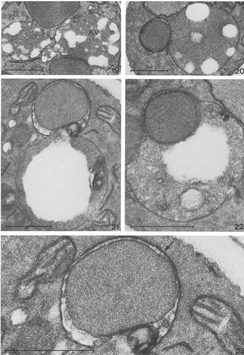
Fig. 19. Detail of a cell showing fusion of two autophagic vacuoles ( D = 0.02 ; t = 60 \text{KMnO}_4 )
