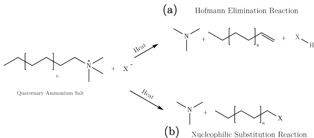
Figure 1: The main mechanisms for degradation (a) Hofmann elimination and (b) nucleophilic substitution 4,6,12 .
