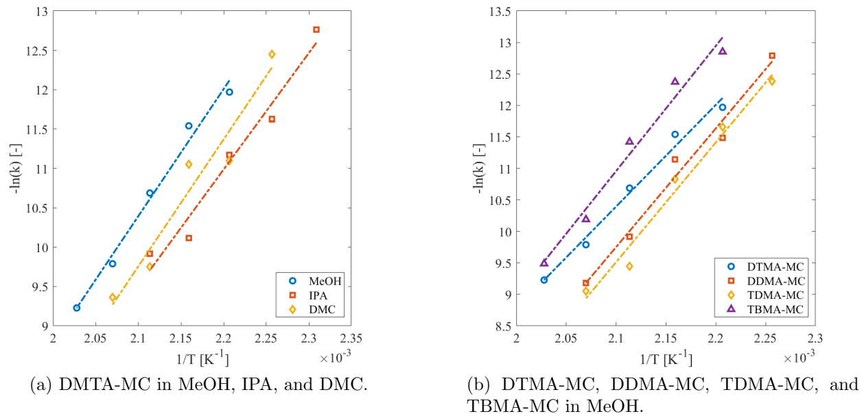
Figure 4: Comparison of all Arrhenius plots for DTMA-MC and MeOH, respectively.
