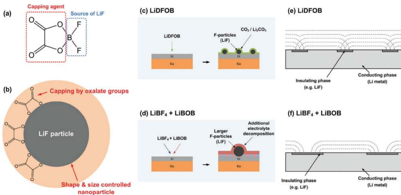
Fig. 15 a, b Proposed mechanisms of LiDFOB acting as a capping agent for LiF nanoparticle generation; c, d models of SEIs from c LiDFOB and d LiBF 4 +LiBOB electrolytes; and e, f schematics of diffusion fields at Li plated from each electrolyte. Each Li plate pos-
