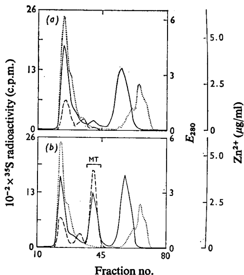
Fig. 1. Separation on Sephadex G-75 of the cytosol from livers of control (a) and zinc-treated (b) rats
