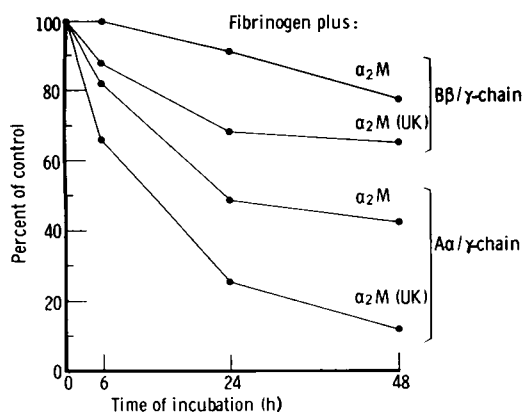
FIGURE 4 Sequential changes in the A \alpha - and B \beta -chains of fibrinogen induced by \alpha_2 -macroglobulin preparations as assessed by densitometric scans. The data are derived from scans of gels 1-6 of Fig. 3 and the corresponding 48-h samples. The ratios of the areas under the A \alpha - and B \beta -position, respectively, to that of the \gamma -chain position is expressed as percent of the ratio found at time 0.
