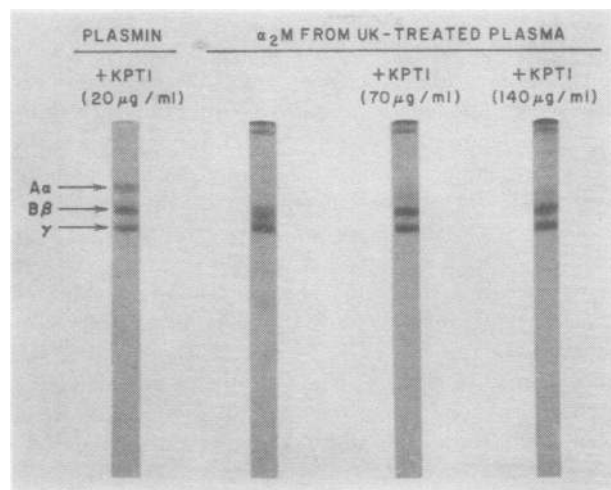
FIGURE 5 SDS-polyacrylamide gel electrophoresis of subunit chains of heat-precipitated fibrinogen after incubation with \alpha_2 -macroglobulin prepared from plasma treated with 500 U urokinase/ml. Fibrinogen (1.6 mg/ml) in the presence or absence of Kunitz pancreatic trypsin inhibitor (KPTI) was incubated at 37°C with human plasmin (0.07 caseinolytic U), or with \alpha_2 -macroglobulin (4.8 mg) prepared from urokinase-treated plasma. Samples were taken at 24 h. The gels referred to in the text are numbered from left to right.
