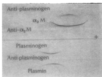
FIGURE 1 Immunoelectrophoretic pattern of \alpha_2 -macroglobulin ( \alpha_2 -M) from urokinase-treated plasma (12 mg/ml, upper slide) diffused against human plasminogen or \alpha_2 -macroglobulin antibody. The immunoelectrophoretic pattern of human plasminogen or urokinase-activated plasmin is shown in the lower slide. The anode is to the right.
