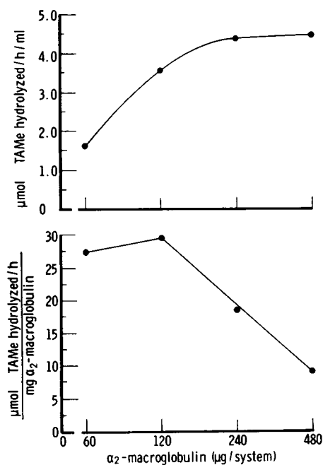
FIGURE 2 The binding of plasmin to \alpha_2 -macroglobulin as determined by the ability of increasing concentrations of \alpha_2 -macroglobulin to protect the TAME esterase activity of a constant concentration of plasmin from inhibition by soybean trypsin inhibitor. Dilutions of \alpha_2 -macroglobulin were added to human plasmin (0.2 caseinolytic U). After 1 min preincubation, 100 \mu g soybean trypsin inhibitor was added, and the mixture was incubated with TAME. The data in the upper graph are plotted to indicate the capacity of \alpha_2 -macroglobulin to protect bound plasmin against inhibition by soybean trypsin inhibitor. The data in the lower graph are plotted to indicate the specific activity of \alpha_2 -macroglobulin.
