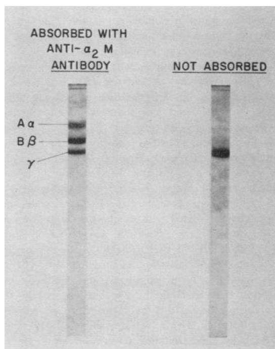
FIGURE 6 SDS-polyacrylamide gel electrophoresis of subunit chains of heat-precipitated fibrinogen after incubation with an antibody-absorbed \alpha_2 -macroglobulin preparation prepared from plasma treated with 500 U urokinase/ml, or with this preparation in the absence of immunoprecipitation. The electrophoretic patterns of samples taken at 48 h are shown in this figure.
