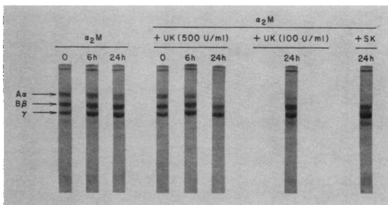
FIGURE 3 SDS-polyacrylamide gel electrophoresis of subunit chains of heat-precipitated fibrinogen after incubation with \alpha_2 -macroglobulin ( \alpha_2 -M) preparations. \alpha_2 -Macroglobulin (4.8 mg/ml), prepared from untreated plasma or from plasma incubated with 100 or 500 U urokinase/ml or 500 U streptokinase/ml, was incubated at 37°C with fibrinogen (1.6 mg/ml) in 0.025 M Tris-HCl buffer, pH 7.5, containing 0.16% sodium citrate and 0.85% sodium chloride. Samples were removed at 0, 6, 24, and 48 h and the fibrinogen precipitated by heating. The precipitate was then redissolved in an SDS urea solution and reduced by treatment with DTT before acrylamide gel electrophoresis. From left to right, fibrinogen incubated with \alpha_2 -macroglobulin from untreated plasma, gels 1, 2, and 3; from plasma treated with 500 U urokinase/ml, gels 4, 5, and 6; from plasma incubated with 100 U urokinase/ml or with 500 U streptokinase/ml, gels 7 and 8, respectively.
