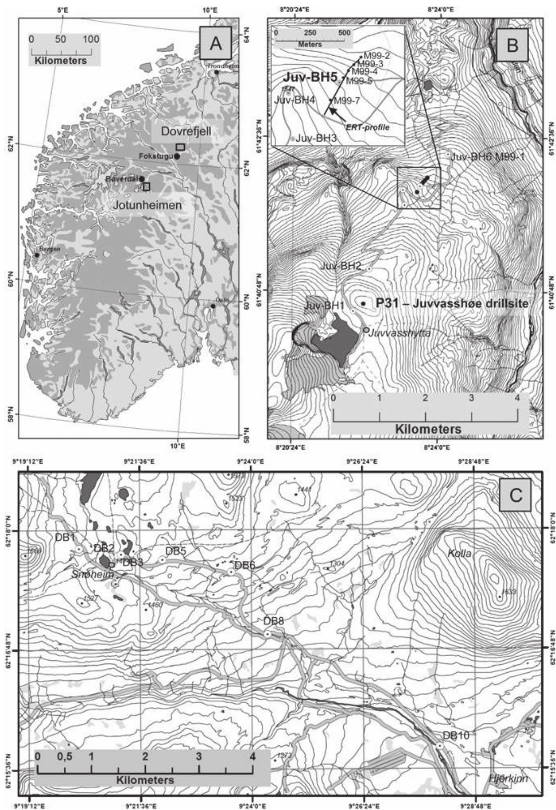
Figure 1 (A) Map of southern Norway showing the location of field sites on and around Juvvasshøe (Jotunheimen) and Snøheim-Hjerkin (Dovrefjell). Fokstugu and Bøverdalen are meteorological stations. (B) Juvvasshøe field site area: JUV-BH1 – 6 are boreholes and M99-1 – 5, 7 are miniature temperature dataloggers. Position of the electrical resistivity tomography (ERT) profile is shown in the inset map. (C) Snøheim-Hjerkin field site: DB1 – 3, 5, 6, 8 and 10 are boreholes.
