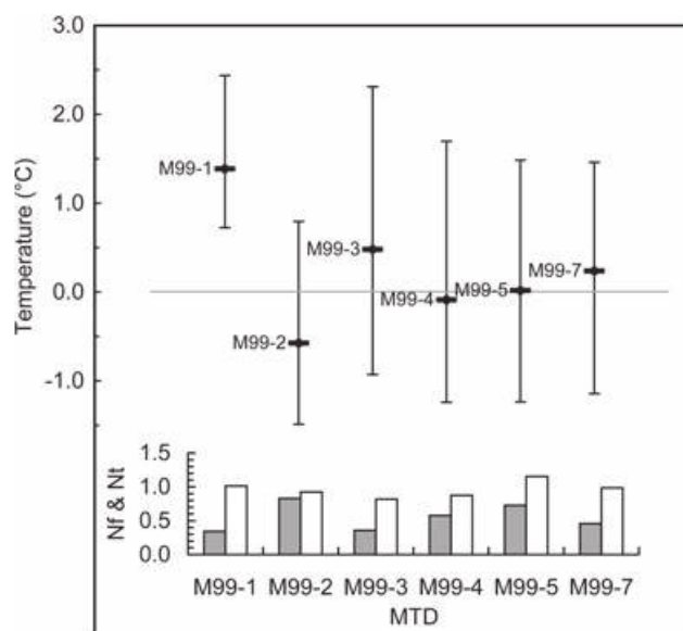
Figure 3 Mean and range of annual mean ground surface temperature for the first four years (August 1999 to May 2003) within the permafrost transition zone along the northeastern slope of Juvvasshøe. N_f -factors (grey bars show N_f , white bars show N_t ; see text for details) for the same period are shown on the lower graph. A detailed description of miniature temperature datalogger (MTD) sites M99-3 and M99-7 and analyses of the first winter 1999–2000 can be found in Figures 11 and 12 in Isaksen et al. (2002).
