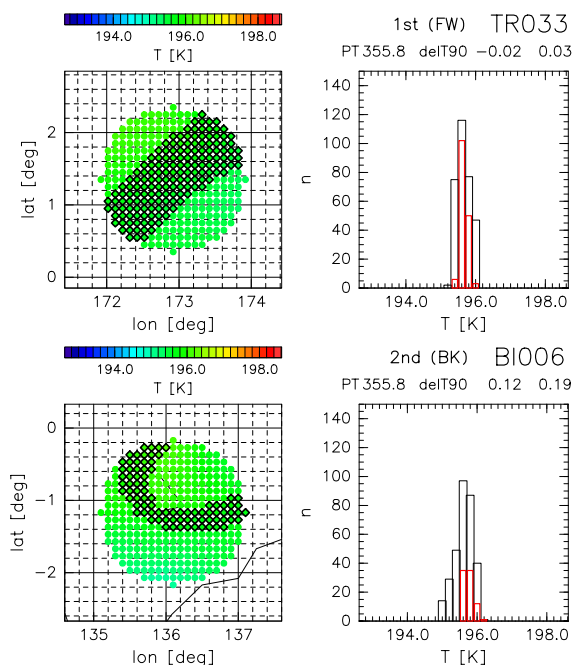
Fig. A1. Representativeness of the match air parcel at Tarawa (top: 05:09 UT, 31 December 2005) and Biak (bottom: 01:49 UT, 6 January 2006). These preliminary matched observations are connected by trajectories at the 355.8 K potential temperature surface. Left: Match air segments (diamonds) superposed on color-coded temperature of the circular area defined by a match radius. Right: Temperature frequency distribution of the whole segments within the circular area defined by a match radius (black bars) and that for match air segments (red bars).
