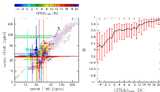
Fig. A4. Examination of convective penetration for the match pairs. Left: Scatter plot of the first versus the second ozone mixing ratios for preliminary matches that passed the screening for “representativeness of match air parcel” color-coded by the value of \langle \delta T_{bb} \rangle_{\min} (see text for details). Right: Dependency of correlation coefficients for ozone mixing ratios between the first and second observations on the value of \langle \delta T_{bb} \rangle_{\min} . The error bars are 99% confidence intervals.
