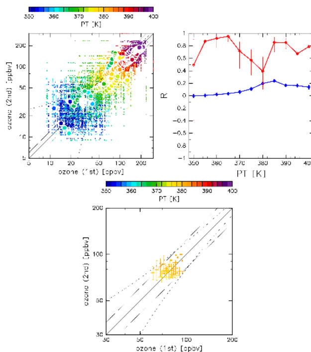
Fig. 3. Left: As for the left panel in Fig. 2 but for preliminary matches for which the time interval between the first and second observations is less than 3 days (large circles). The small dots represent all of the possible paired (see the text for details on the pairing procedure) observations (to reduce clutter, not all data are shown). Center: Correlation coefficients calculated for every 5 K of potential temperature (with \pm 2.5 K bins) for the preliminary matches (red) and for all possible paired observations (blue). Error bars are 90 % confidence intervals. Right: As for the large circles in the left panel but for pairs at altitudes from 377.5 K to 382.5 K.
