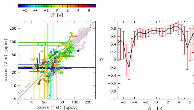
Fig. A6. As for Fig. A5 but for examining the consistency between sonde data and the analysis field.
