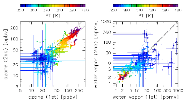
Fig. 2. Scatter plots showing the first (abscissa) versus the second observed values (ordinate) of ozone (left) and water vapor (right) mixing ratios for all preliminary matches connected by match air parcel. Color indicates the potential temperature. Bars in both panels indicate the uncertainties estimated by Hasebe et al. (2013), a companion paper to the present study. The dashed lines oriented parallel to the diagonal in the left panel indicate a difference of \pm 20\% between the paired observations, and the dotted curves indicate the range of \pm 20 ppbv difference for the paired ozone mixing ratio. These are the thresholds of acceptable difference used in this study (see the last part of Sect. 3.3). Lines in the right panel indicate the accuracy of water vapor measurements; i.e., \pm 10\% (dashed lines) and \pm 1 ppmv (dotted lines) (see Sect. 2). Note that the water vapor data measured by the Snow White hygrometers are not plotted above 360 K by their performance problem (see Sect. 2).
