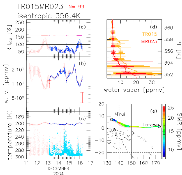
Fig. 6. As for Fig. 5 but for the match that advected from Tarawa (03:48 UT, 13 December 2004) to Mirai (05:17 UT on 16 December 2004) at the 356.4 K potential temperature surface with an advection time of about 3 days.
