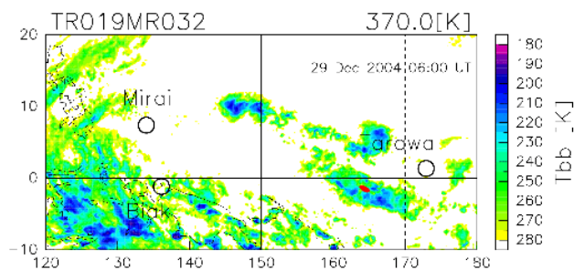
Fig. A3. Match air segments (red area at \sim 2^\circ S, \sim 164^\circ E) similar to the red dots in Fig. 1 superposed on the distribution of T_{bb} (color) at 06:00 UT on 29 December 2004. The black circles show the circles of the match radius ( 1^\circ ) centered at individual observational stations.
