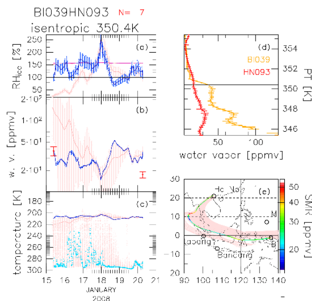
Fig. 7. As for Fig. 5 but for the match that advected from Biak (09:46 UT, 15 January 2008) to Hanoi (06:45 UT, 20 January 2008) at the 350.4 K potential temperature surface with an advection time of about 5 days.
