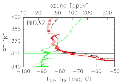
Fig. 8. Vertical profiles of frost point temperature (red), temperature (black), and ozone mixing ratio (green) observed at Biak (04:35 UT, 16 January 2007). The horizontal bars show the uncertainties of sonde measurements estimated by Hasebe et al. (2013) (see appendix A in their paper).
