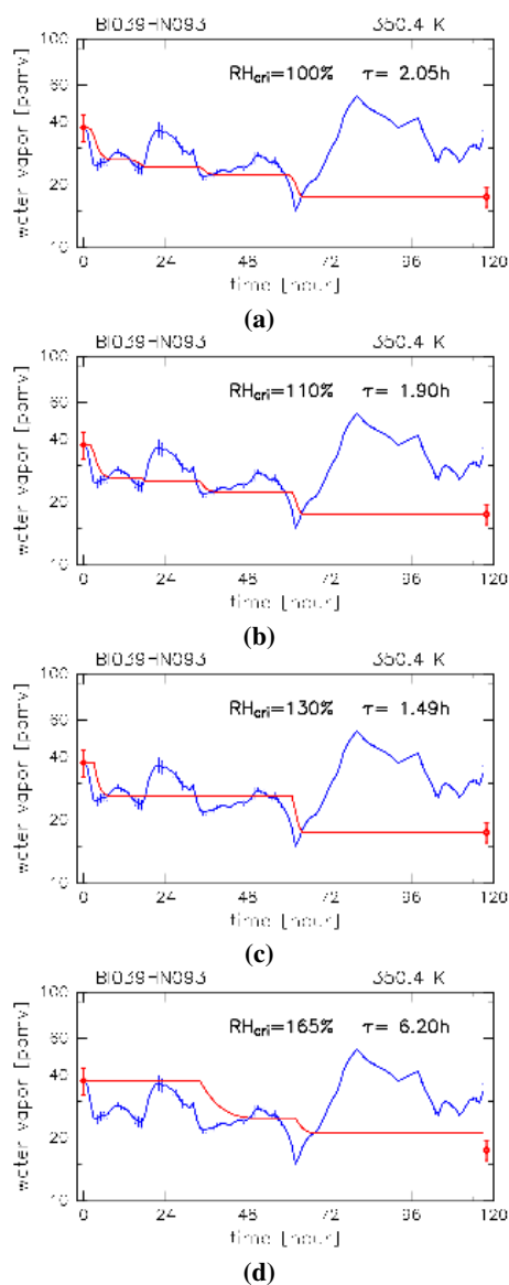
Fig. 10. Dehydration scenarios showing the time evolution of the water vapor mixing ratio of the air mass (red line) and exposed SMR (blue line) estimated from the match case shown in Fig. 7. The value of \tau stated in each panel is the estimated relaxation time of condensation for the assumed values of RH_{\text{cri}} , which are (a) 100 %, (b) 110 %, (c) 130 %, and (d) 165 %.
