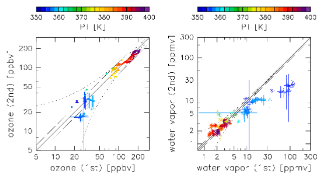
Fig. 4. As for Fig. 2 but for matches identified after applying all of the screening procedures (Sect. 3.3). In the right panel, the axes are modified compared with Fig. 2 and the symbols refer to the hygrometers, i.e., crosses, triangles, and circles indicate paired observations by CFH and CFH (for the first and second observations, respectively), CFH and SW, and SW and SW, respectively.
