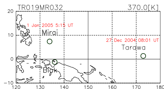
Fig. 1. Example of a cluster of trajectories leaving Tarawa. The blue and red dots are the whole segments calculated from the circled region with a match radius ( 1^\circ ) centered at Tarawa. Only the red dots are included in both the first and second circular areas (i.e., those centered at Tarawa and Mirai , respectively); therefore, they represent a match air parcel (see text for details). The footprints are drawn every 24 h. The air parcel observed over Tarawa on 27 December 2004 (first observation) was observed again (second observation) over Mirai after about 5 days.
