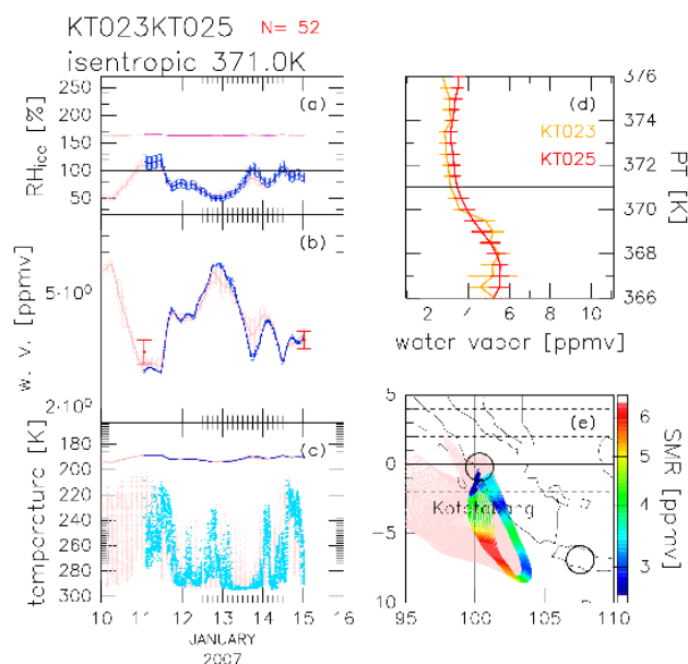
Fig. 5. Meteorological conditions of the match advecting from Kototabang (01:42 UT, 11 January 2007) to Kototabang (00:37 UT, 15 January 2007) on the 371.0 K potential temperature surface. Those times correspond to the times of observations, i.e., 50 min after each launch (see Sect. 3.2). Vertical profiles of water vapor measured at the first (orange) and second (red) observations, along with estimates of errors, are shown in (d). The figure shows the time evolutions of (a) relative humidity over ice ( RH_{ice} ) on the assumption that the water vapor amount is unchanged from the first measurement, along with the uncertainties (blue) and the homogeneous freezing threshold ( RH_{hom} ; purple); (b) saturation water vapor mixing ratio (SMR; blue line); (c) temperature (blue line) and equivalent black body temperature ( T_{bb} ; light blue dots); and (e) trajectories of the match air parcel, color coded by SMR history. In (b), the superposed vertical bars in red are the water vapor mixing ratio measured at the match altitude (horizontal black line in (d)). Meteorological data are from ECMWF, and T_{bb} values are derived from MTSAT-1R/GOES-9 IR images. For (a), (b), (c), and (e) each meteorological value for the match air mass is superposed on that for the whole segments calculated from the circular region centered at the second observation (pink shading).
