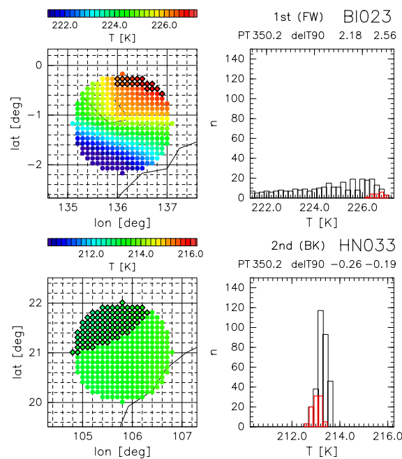
Fig. A2. As for Fig. A1 but for the preliminary match at Biak (top: 22:50 UT, 18 January 2006) and Hanoi (bottom: 06:57 UT, 21 January 2006) on the 350.2 K potential temperature surface.
