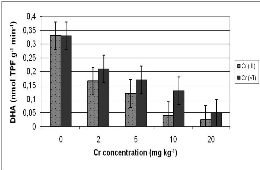
Figure 15. The variations of DHA in Eutric Cambisol at different Cr (III) and Cr (VI) concentrations (according to Stępniewska & Wolińska, 2004). Averaged values of three replicates with standard deviations are presented
