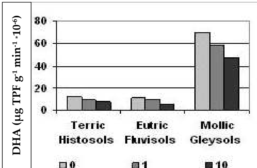
Figure 12. Mean DHA in Terric Histosols , Eutric Fluvisols and Mollic Gleysols , in three combinations of Glyphosate doses: 0-control; 1-1 \mu\text{g} \text{g}^{-1} ; 10-10 \mu\text{g} \text{g}^{-1} (according to Bennicelli et al., 2009)
