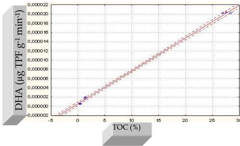
Figure 5. Relationship between DHA and TOC content in the Mollic Gleysol ( n=9 , r=0.99^{***} ), according to Wolińska & Stepniwska (unpublished data)
