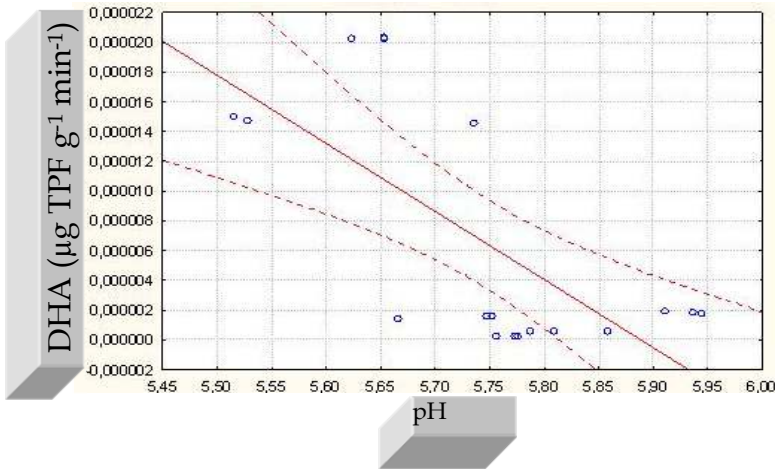
Figure 6. Relationship between DHA and pH values in the Mollic Gleysol ( n=18 , r=-0.70^{**} ), according to Wolińska & Stepniewska (unpublished data)
