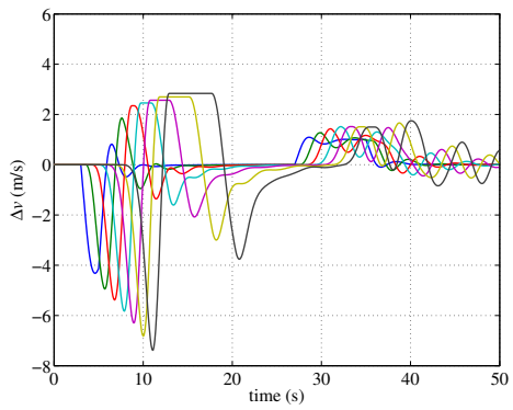
(c) \tau^S = 0.5 s without compensation
