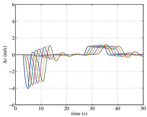
(e) \tau^A = 0.4 s without compensation
