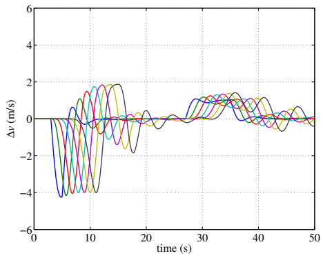
(g) \tau^A = 0.5 s without compensation
