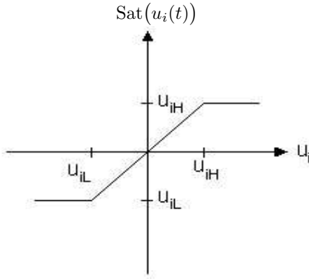
Fig. 1. Saturation function.
