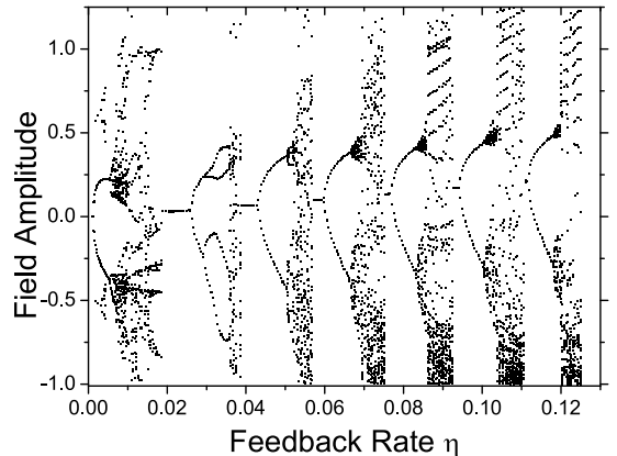
FIG. 5: Bifurcation diagram of the field amplitude; plotted are \max(\frac{R}{\sqrt{P}} - 1.0) and \min(\frac{R}{\sqrt{P}} - 1.0) as a function of feedback strength \eta for the parameter values T = 1710 , \alpha = 5.0 , P = 0.8 , \tau = 70 , and C_p = 0.0 .
