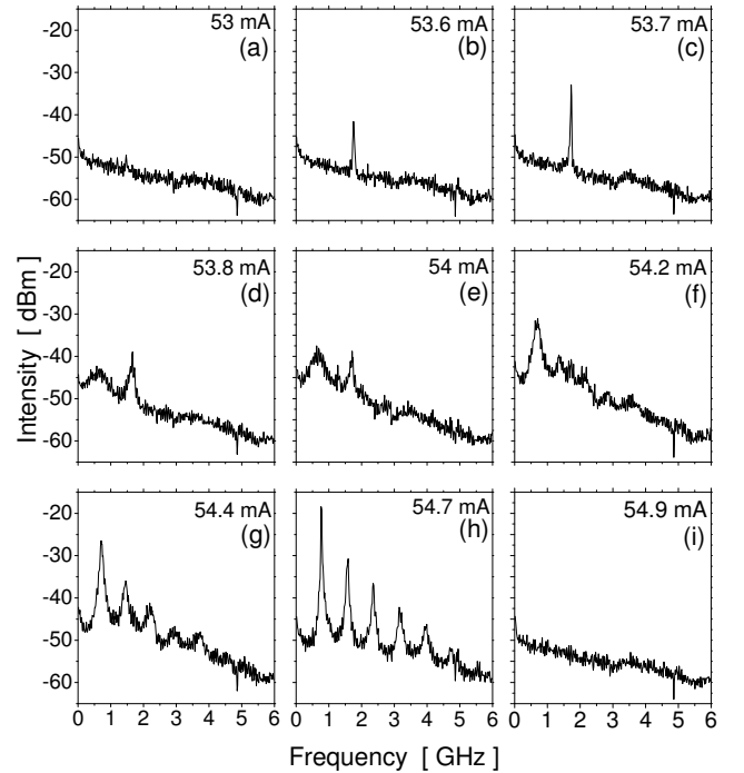
FIG. 4: One cycle of the repeating dynamical scenario characterized by the rf-spectra of the laser emission. The external cavity length is 1.1 cm and the threshold reduction 11.5%. The injection current is indicated on each panel.
