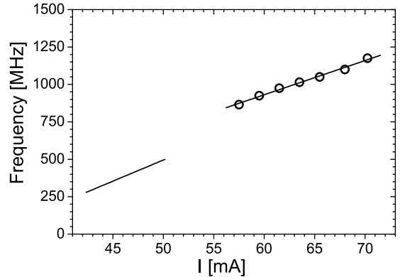
FIG. 3: Dependence of the RPP envelope frequency \nu_{RPP} on the injection current. The squares represent the results for an external cavity with \nu_{EC} = 4.1 GHz, the circles represent the data for the cavity with \nu_{EC} = 14 GHz. The lines are linear fits to the experimental data.
