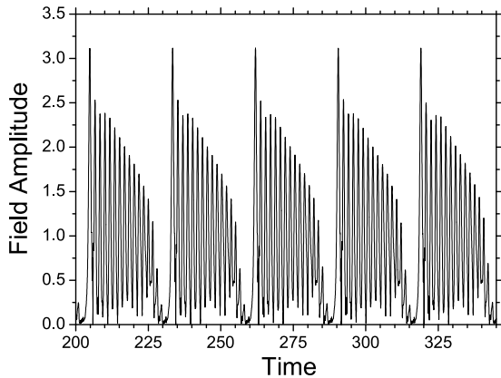
FIG. 6: Time series of the amplitude of the RPP. The time has been normalized to the relaxation frequency of the laser, \omega_r = \sqrt{2P/T} . The parameter values are T = 1710 , \alpha = 5.0 , P = 0.8 , \tau = 70 , C_p = \pi , and \eta = 0.115 .
