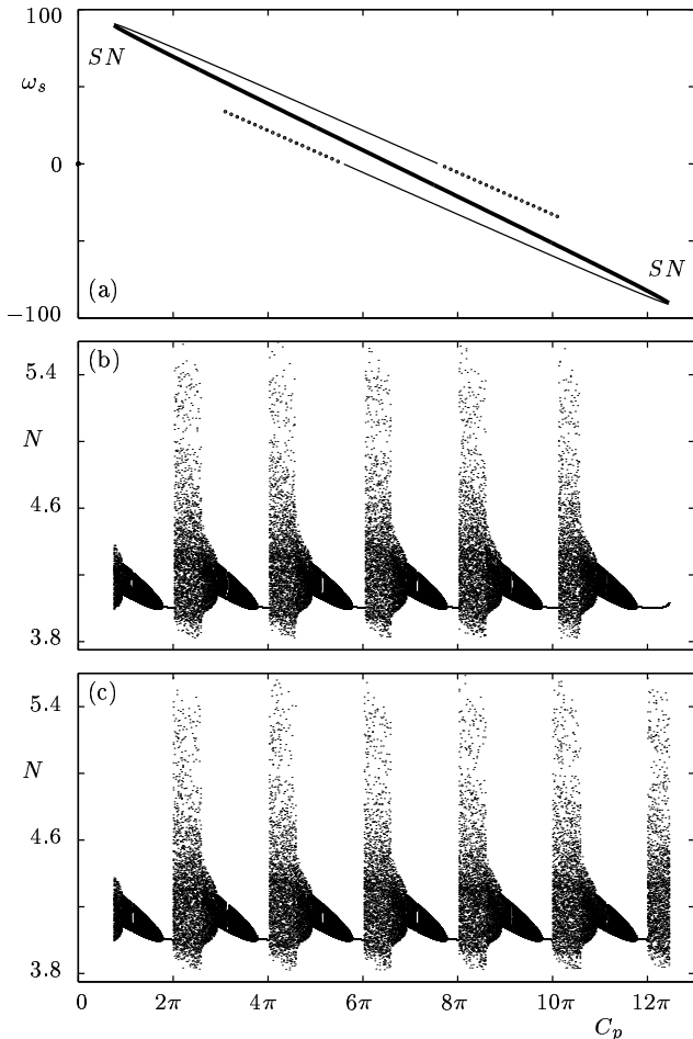
FIG. 11: Continuation of the mode/anti-mode pair from creation to annihilation ‘unwrapped’ and plotted over its entire range of phase C_p (a), and intersections of the attractors (b) and (c) to which the first and second branch, respectively, of the (strong) unstable manifold of the saddle point (anti-mode and thick curve in (a)) converge to. The other parameters are as in Table I.
