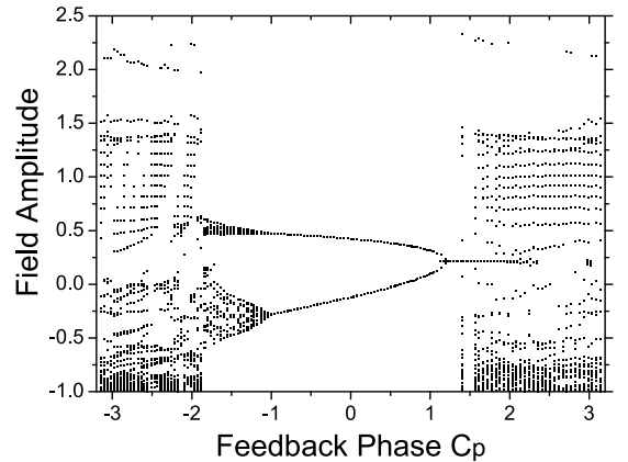
FIG. 7: Bifurcation diagram of the field amplitude, where we plotted \max(\frac{R}{\sqrt{P}} - 1.0) and \min(\frac{R}{\sqrt{P}} - 1.0) as a function of C_p \in [-\pi, \pi] at \eta = 0.115 . The other parameters are as in Fig. 6.
