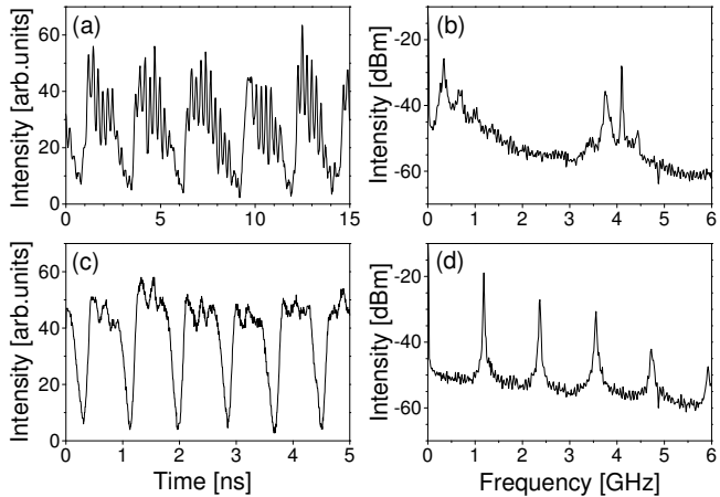
FIG. 2: Pulse Packages in the intensity dynamics of a semiconductor laser operating in the Short Cavity Regime. The time series in panel (a) and the corresponding rf-spectrum in panel (b) were recorded for an external cavity length of 3.7 cm and an injection current of 1.08 I_{th,sol} ; the external cavity round-trip oscillations of \nu_{EC}=4.1 GHz are fully resolved in the time series. The time series in panel (c) and the rf-spectrum panel (d) were recorded for an external cavity length of 1.1 cm and an injection current of 1.8 I_{th,sol} ; the external cavity round-trip oscillations of approximately \nu_{EC}=14 GHz are not fully resolved in the time series.
