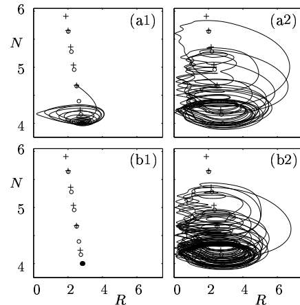
FIG. 13: Bistability region near the MGM: The two branches of the unstable manifold of one saddle ECM, shown in panels (a1) and (a2), converge to the MGM (b1) and the RPP attractor (b2), respectively. Here C_p = 31.494 and the other parameters are as in Table I.
