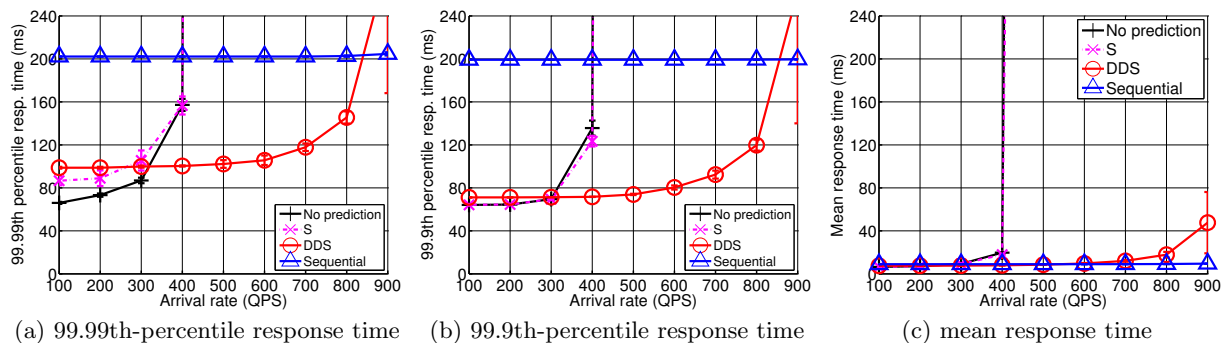
Figure 5: Response time of sequential and three parallel query execution approaches at ISN.
