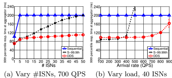
Figure 8: 99th-percentile latency at an aggregator.
