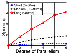
Figure 4: Parallelization efficiency of short, medium and long-running queries.
