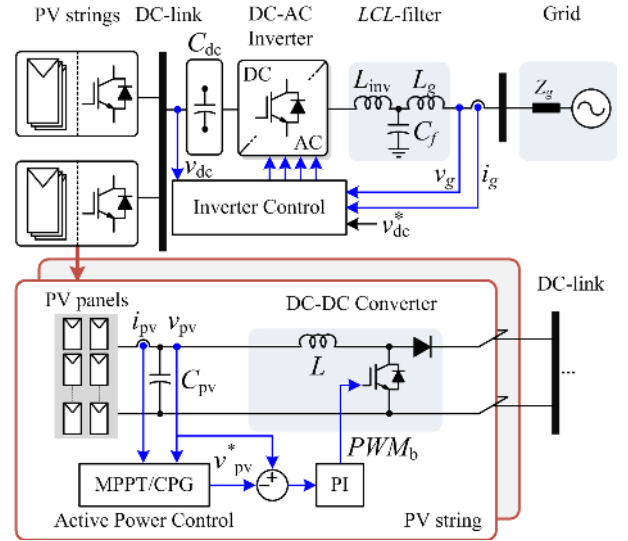
Fig. 4. System configuration and control structure of multi-string grid-connected PV inverters [29].
