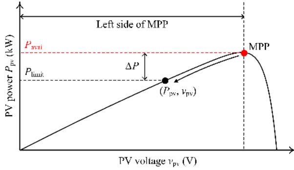
Fig. 3. Power-voltage characteristic of the PV panels with the operating point at the power limit P_{\text{limit}} , where MPP is the maximum power point.
