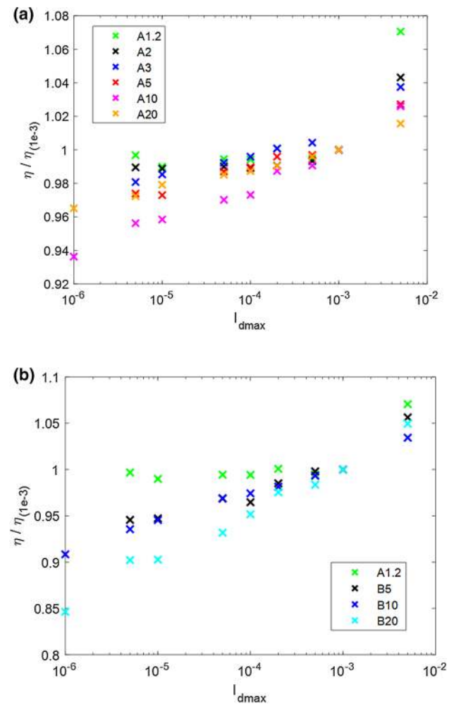
Fig. 9 Effect of I_{d\max} on stress ratio at \varepsilon_1 = 2\% . Results are normalized by the response at I_{d\max} = 1 \times 10^{-3} : a series A; b series B
