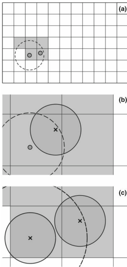
Fig. 3 2D schematic showing interactions between different particle types: a small–small interactions; b small–large interactions; c large–large interactions
