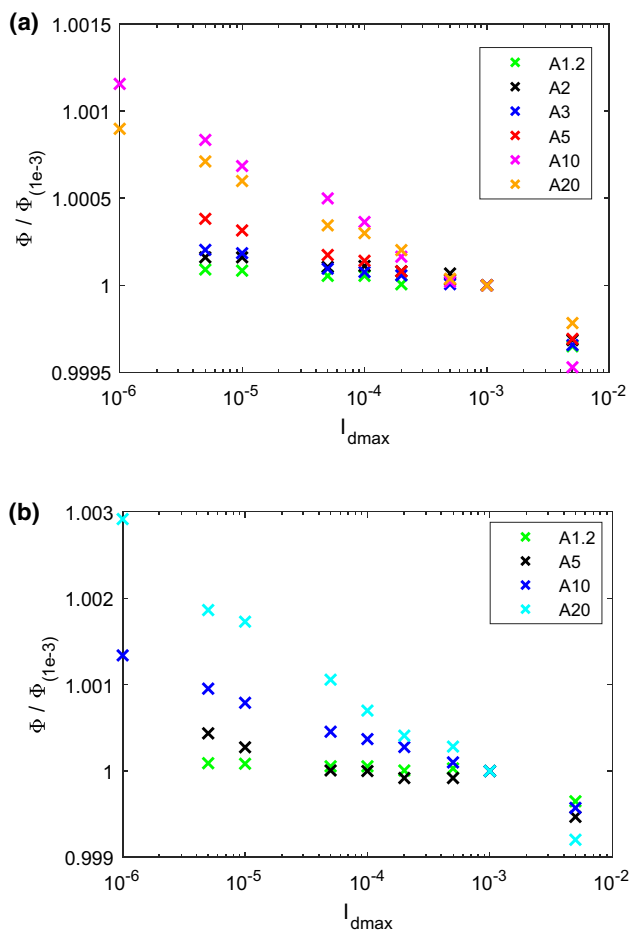
Fig. 10 Effect of I_{dmax} on solid packing fraction at \varepsilon_1 = 2\% . Results are normalized by the response at I_{dmax} = 1 \times 10^{-3} : a series A; b series B
