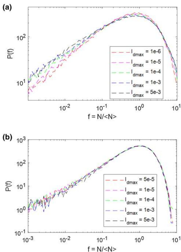
Fig. 12 Probability density functions of normal contact force, N , normalized by mean normal contact force, \langle N \rangle . a Sample B20; b sample A1.2
