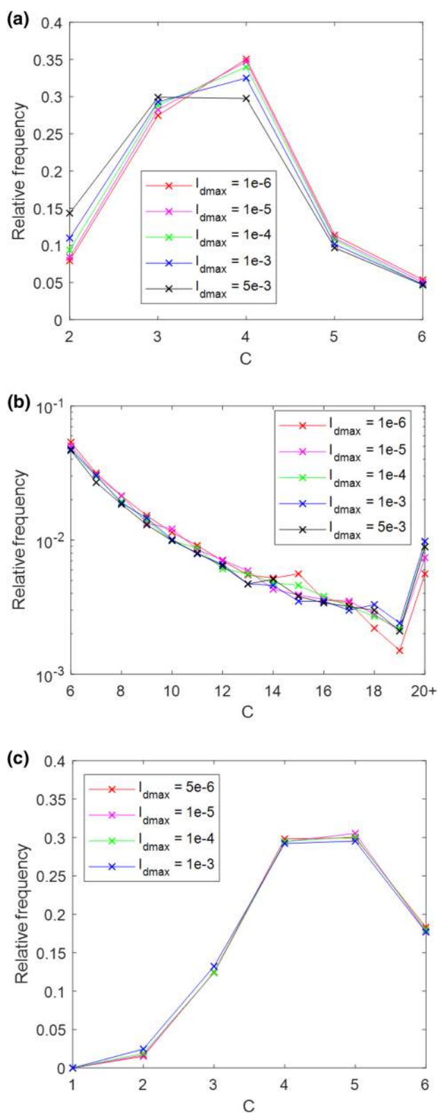
Fig. 13 Relative frequency plot of connectivity, C : a sample B20, contacts C \leq 6 (note linear y-scale); b sample B20, contacts C \geq 6 (note log y-scale); c sample A1.2, contacts C \leq 6
