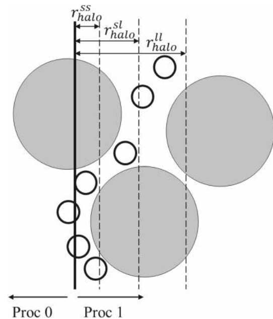
Fig. 4 Schematic of hierarchical stencil inter-processor communication (adapted from [11]). Halos of different dimensions are adopted depending on the interaction type (i.e., large–large, small–large or small–small)
