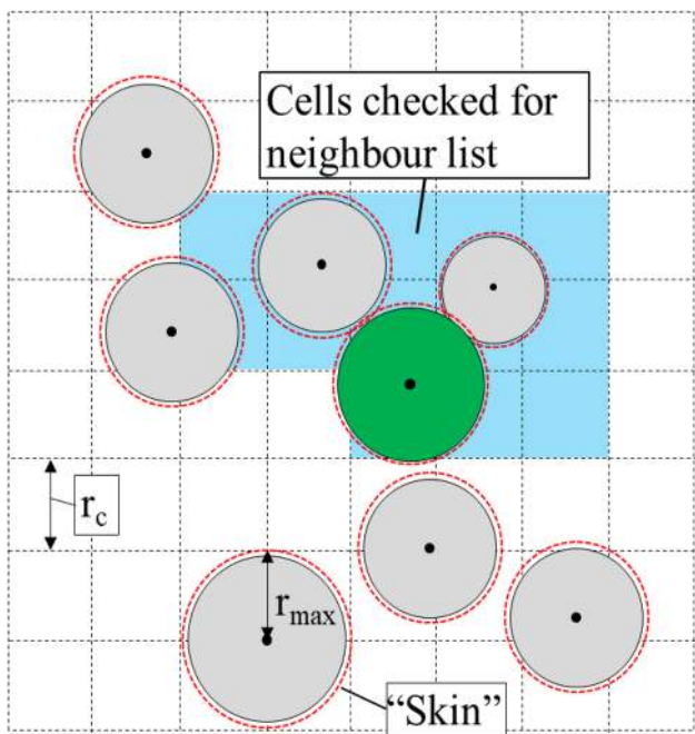
Fig. 1 Schematic showing link-cell contact detection in LAMMPS, where r_{\max} is the maximum particle radius, and r_c is the cell dimension. r_c = r_{\max} + r_{\text{skin}} where r_{\text{skin}} is the skin distance
