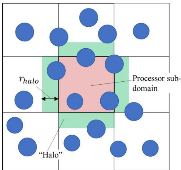
Fig. 2 2D schematic of inter-processor communication in LAMMPS. Particle information within the halo of dimension r_{\text{halo}} must be communicated to the processor subdomain at every timestep
