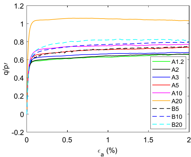
Fig. 6 Stress ratio behavior during shearing at I_{d\max} = 1 \times 10^{-3}
