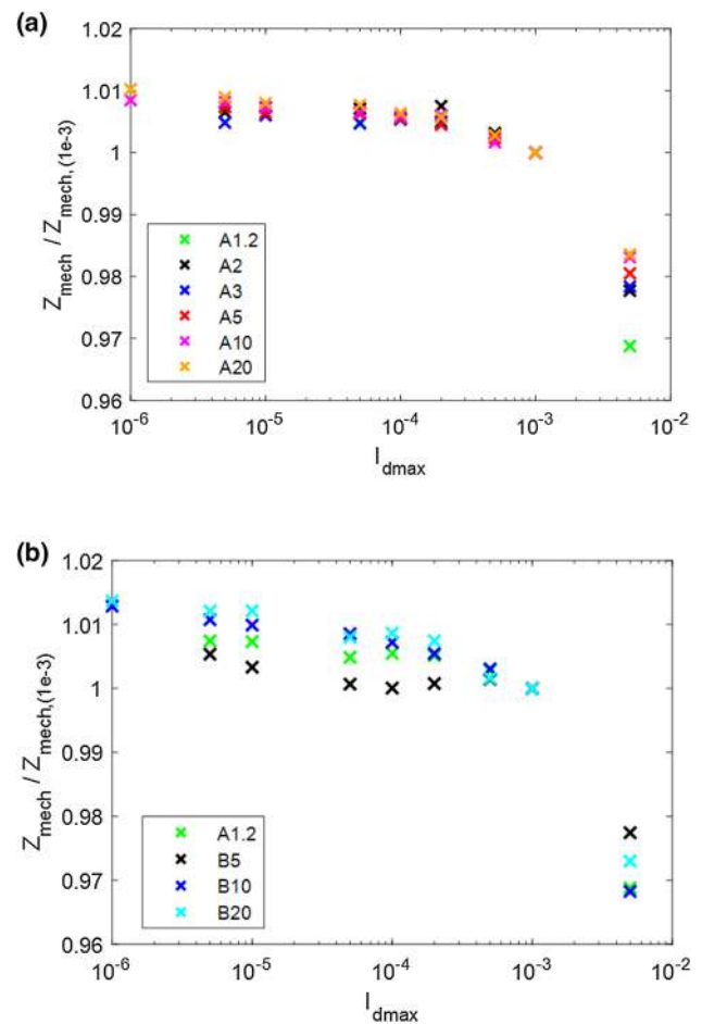
Fig. 11 Effect of I_{dmax} on mechanical coordination number at \varepsilon_1 = 2\% . Results are normalized by the response at I_{dmax} = 1 \times 10^{-3} : a series A; b series B
