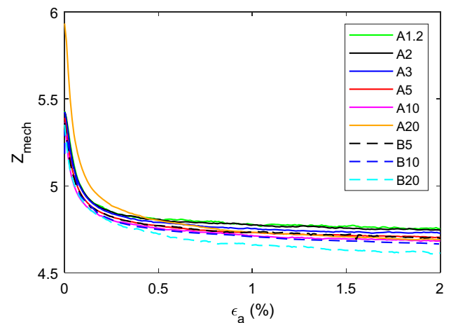
Fig. 8 Mechanical coordination number during shearing at I_{d\max} = 1 \times 10^{-3}
