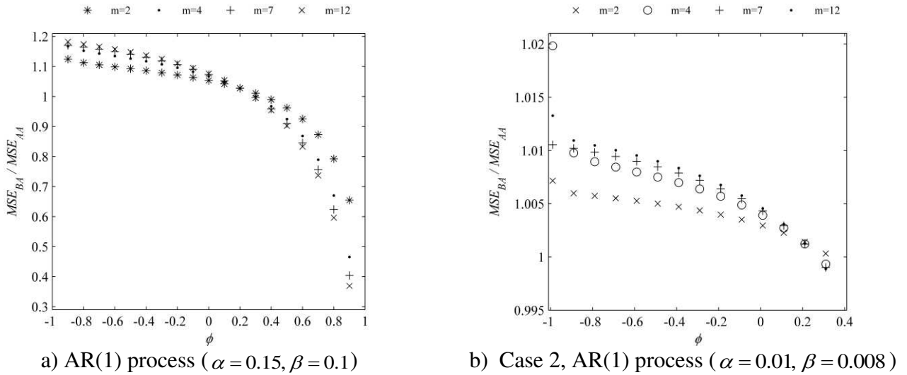
Figure 3. MSE ratio for different values of m
