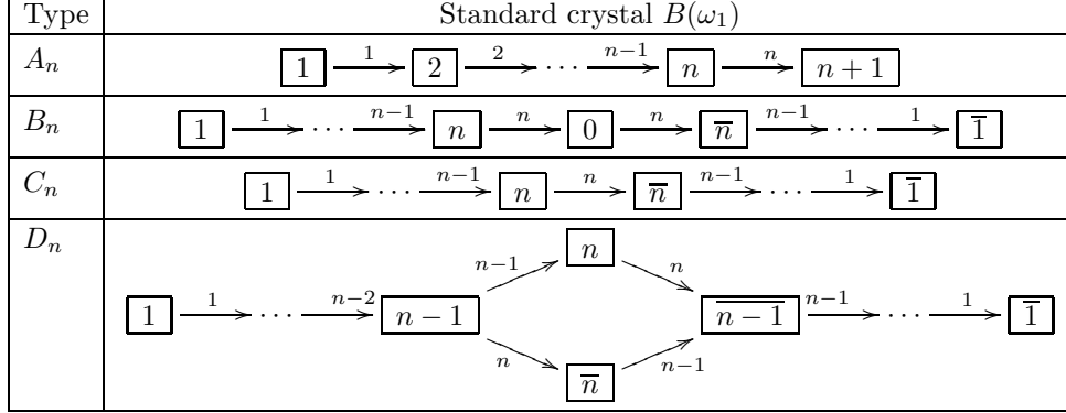
FIGURE 2. Standard crystals. The boxes represent the vertices of the crystal, and each arrow labeled i shows the action of f_i .
