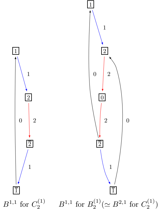
FIGURE 1. Examples of perfect and non-perfect U'_q(\mathfrak{g}) crystals. One can verify that the crystal on the right is perfect of level 1, and the crystal on the left is not perfect of any level. These crystals are both KR crystals, as indicated, and the vertices are indexed by KN tableaux as in Section 3.1. In fact, all known finite U'_q(\mathfrak{g}) crystals are KR crystals or tensor products of KR crystals.
