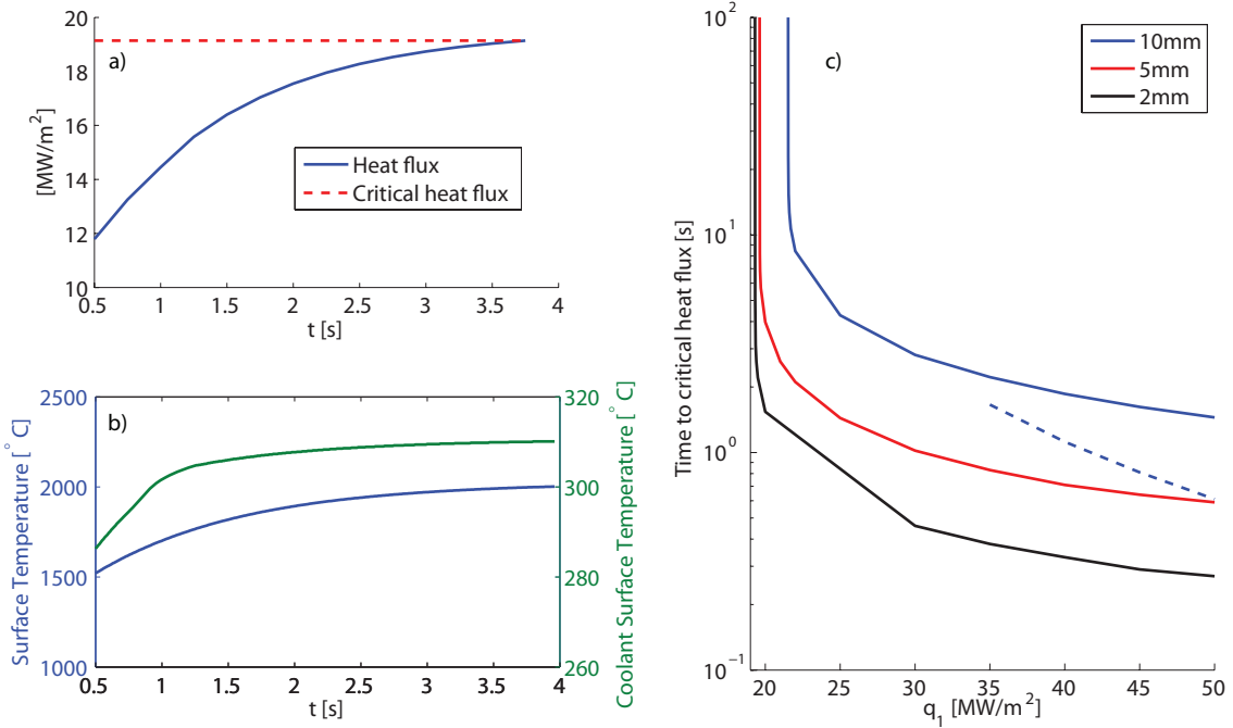
Figure 1. Results of RACLETTE calculations with mass flow rate 8 \times 10^3 \text{ kg/m}^2/\text{s} , pressure 4MPa, pipe inlet temperature 200^\circ\text{C} and turbulence promotion factor 1.9 (swirl tube): a) Heat flux as a function of time and critical heat flux at the interface between Cu and the coolant after a sudden increase of the target power flux density to 20 \text{ MW/m}^2 at t = 0\text{s} (W thickness: 5mm). b) Evolution of temperatures at the surface and at the interface between Cu and coolant. c) Time until the heat flux reaches the critical heat flux as function of target power flux density and W thickness. The dashed line shows the surface melt limit for the cases, where it is more restrictive (W thickness: 10mm).
