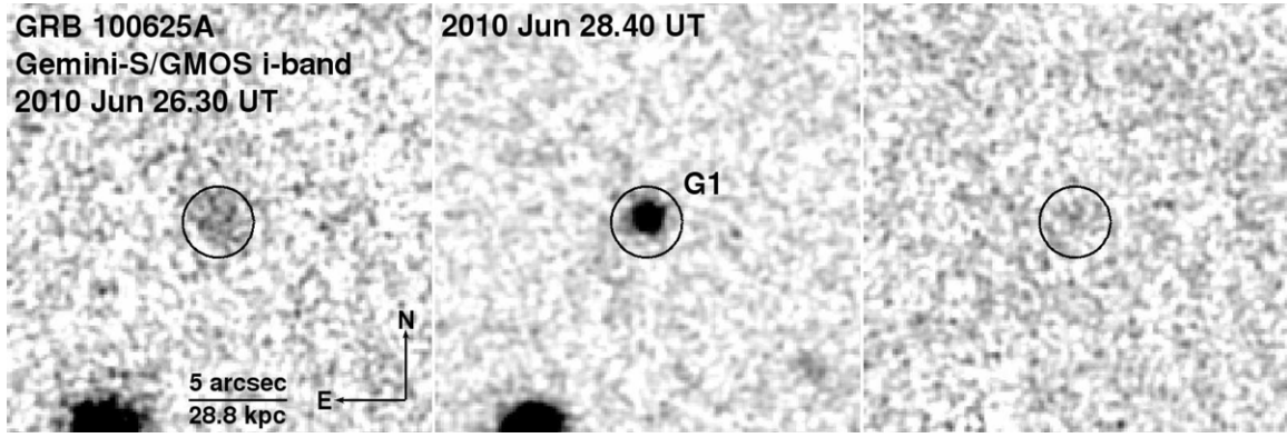
Figure 2. Gemini-South/GMOS i -band observations of GRB 100625A. The XRT error circle has a radius of 1''.8 (90% containment; black). Images are smoothed with a 2-pixel Gaussian. Left: \delta t = 0.53 days in poor seeing conditions ( \theta_{\text{FWHM}} = 1''.9 ) with a faint host detection. Center: \delta t = 2.63 days with 0''.9 seeing. Right: digital image subtraction of the two epochs reveals no afterglow to a 3\sigma limit of i \gtrsim 22.7 mag. The host galaxy is marked as G1.
