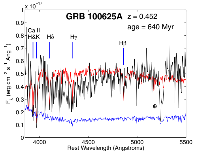
Figure 7. LDSS3 spectrum of the early-type host galaxy of GRB 100625A, binned with a 3-pixel boxcar (black: data; blue: error spectrum). Also shown is the best-fit SSP template (red; Bruzual & Charlot 2003) with a stellar population age of 640 Myr at a redshift of z = 0.452 \pm 0.002 . Fits are performed on the unbinned data. The locations of the Balmer absorption lines and Ca II H&K are labeled.
