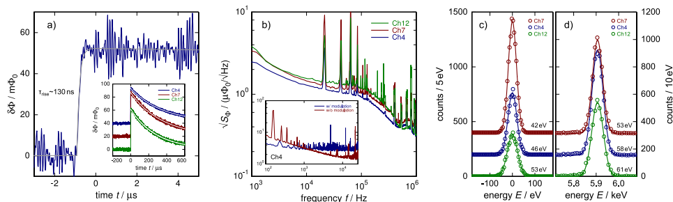
FIG. 4. (a) Signal rise of a raw signal of channel 4. The grey line is a fit assuming an exponential time dependence. The inset shows raw signals for channels 4, 7, and 12. The white solid lines show fits to the signal decay assuming a single exponential time dependence. (b) Measured noise spectra of channels 4, 7, and 12 as calculated from untriggered baselines. The low-pass characteristic at high frequencies is due to a low-pass filter. The inset shows noise spectra of channel 4 that were acquired with and without flux ramp modulation. (c) Measured baseline spectra as well as (d) Mn K_\alpha fluorescence spectra of channels 4, 7, and 12. The solid lines show a Gaussian energy distribution with a width given in the figure.
