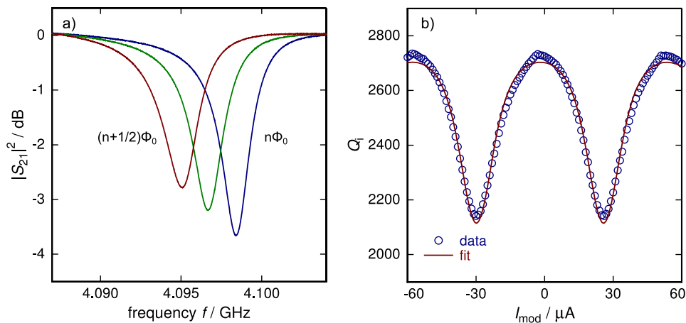
FIG. 3. (a) Transmission curve |S_{21}|^2(f) of channel 4 for three different values of the magnetic flux threading the SQUID loop. (b) Magnetic flux dependence of the intrinsic quality factor of the resonator of channel 4 as well as a fit assuming a small subgap resistance of the Josephson junction.
