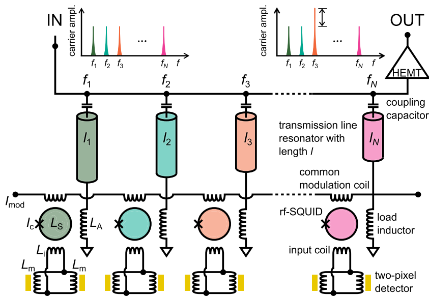
FIG. 1. Schematic circuit diagram of the 64 pixel MMC detector array that is read out by an on-chip, integrated microwave SQUID multiplexer. Each detector consists of two meander-shaped pickup coils that are equipped with a planar paramagnetic temperature sensor. Both pickup coils are connected in parallel with the input coil of the associated non-hysteretic rf-SQUID via superconducting striplines. The insets show as an example the sent and received frequency combs when performing an amplitude based \mu MUX readout and assuming a detector event in channel 3. More details on the actual detector and SQUID geometry can be found in Fig. 2.
