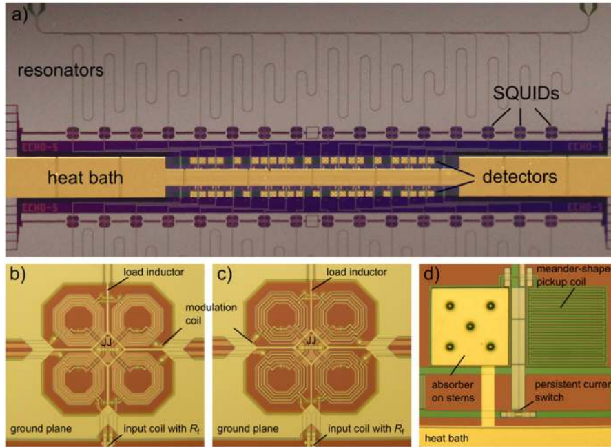
FIG. 2. Photographs of the detector array with on-chip, integrated \mu MUX: a) Overview of the upper two-thirds of the device. b) SQUID formed by four continuous washers connected in parallel. c) SQUID formed by four slotted washers connected in parallel. d) Two-pixel detector for which only one meander-shaped pickup coil is equipped with a temperature sensor and an absorber.
